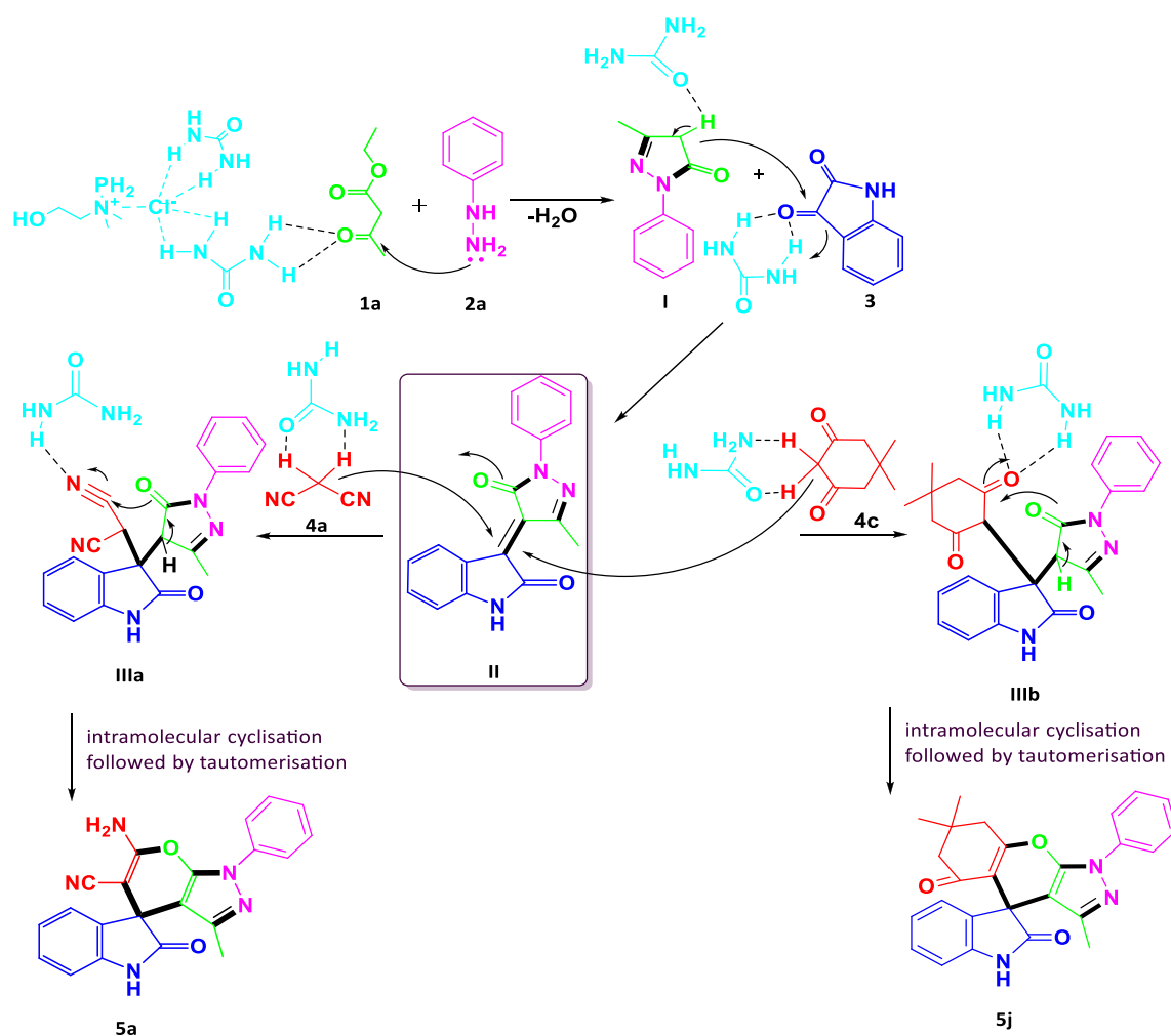
Scheme 2. Probable mechanism of spirooxindole derivatives synthesis.
