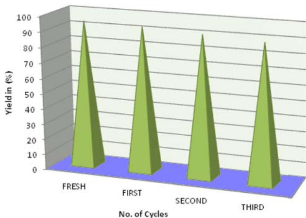
Figure 3. Recycling studies of deep eutectic mixture of (urea:ChCl) in reaction of ethylacetoacetate 1a , phenyl hydrazine 2a , isatin 3a and malonitrile 4a .
