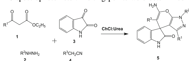
Scheme 1. Synthesis of spirooxindoles in DES.
