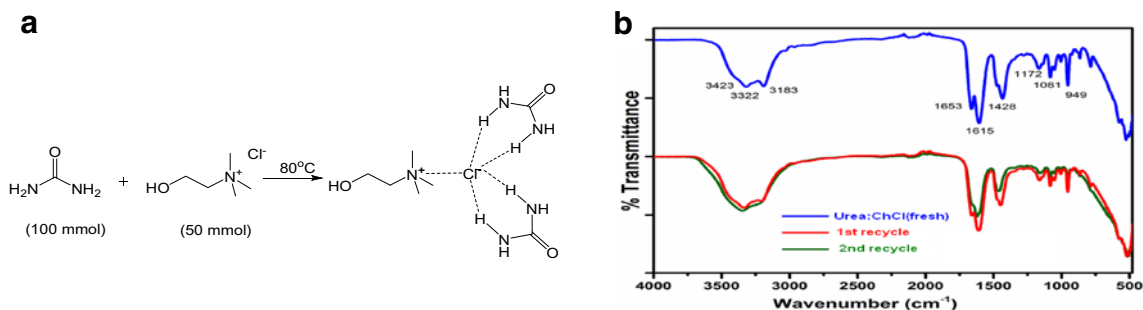
Figure 2. (a) Deep eutectic solvent preparation from urea and ChCl in 2:1 ratio. (b) The FT-IR spectra of freshly prepared Urea:ChCl (2:1) and the 1st recycled and 2nd recycled Urea:ChCl (2:1).
