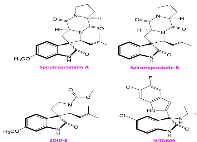
Figure 1. Examples of natural products and synthetic therapeutic agents containing a spirooxindole core.
