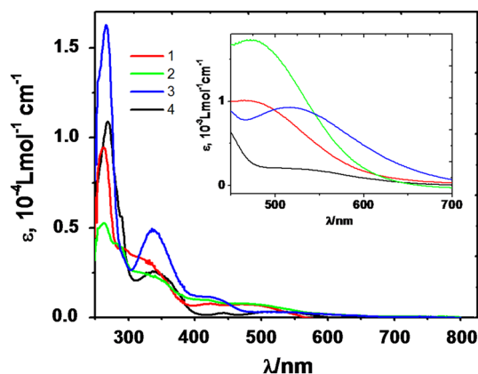
Figure 1. The UV-visible spectrum of the complexes 1–4 in DMF-H 2 O (10% v/v DMF:H 2 O) with the inset showing their d–d bands.
