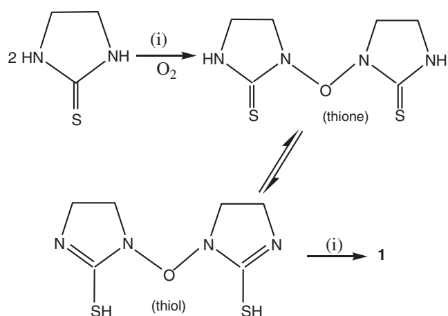
Scheme 2. (i) \text{PdCl}_2(\text{PPh}_3)_2 , \text{Et}_3\text{N} .
