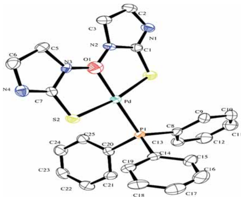
Figure 1. ORTEP diagram for complex 1 at 30% probability. Hydrogens and the solvent molecule have been removed for clarity. Selected bond lengths/Å and angles/°: P1–Pd, 2.3393(10); S1–Pd, 2.2866(12); S2–Pd, 2.3018(12); Pd–O1, 2.016(4); N2–O1, 1.344(5); N3–O1, 1.346(5); C1–S1, 1.739(4); C7–S2, 1.739(4); S1–Pd–S2, 169.60(4); O1–Pd–P1, 177.58(11); S1–Pd–P1, 95.81(4); S2–Pd–P1, 94.14(4); O1–Pd–S1, 85.12(12); O1–Pd–S2, 85.06(12).
