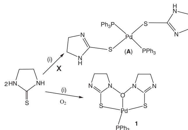
Scheme 1. (i) PdCl 2 (PPh 3 ) 2 , Et 3 N.
