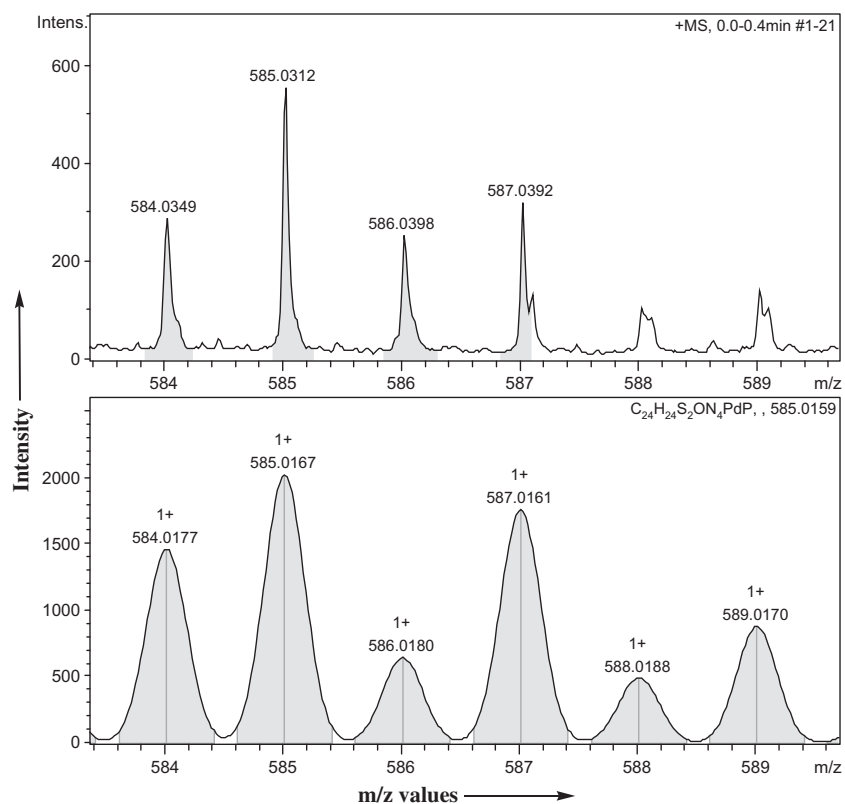
Figure 2. Isotopic pattern of molecular species, [M+H]^+ : (above) observed, m/z = 585.03 , (below) calcd. 585.02).
