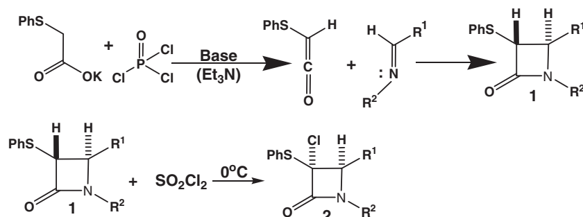
Scheme 1. Synthesis of starting compounds-3-phenylthioazetididin-2-ones 1 & 3-chloro-3-phenylthioazetididin-2-ones 2 .
