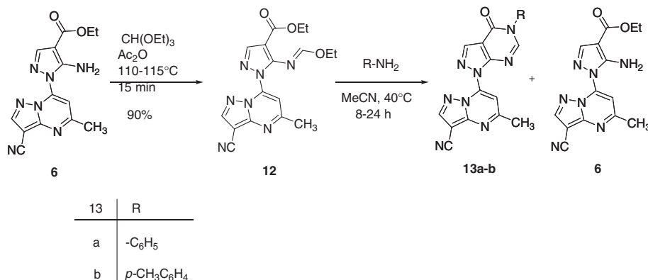
Scheme 4. Synthesis of pyrazolo[3,4- d ]pyrimidines- pyrazolo[1,5- a ]pyrimidine 13a-b .
