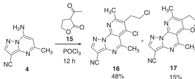
Scheme 6. Synthesis of pyrazolo-pyrido-pyrimidine 16 and dihydrofuro-pyridopyrazolo-pyrimidine 17 .
