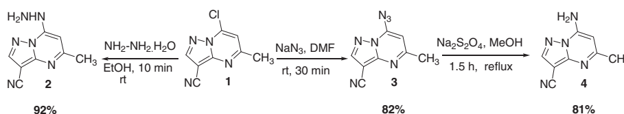
Scheme 1. Synthesis of 7-hydrazinyl-5-methylpyrazolo[1,5- a ]pyrimidine-3-carbonitrile 2 and 7-amino-5-methylpyrazolo[1,5- a ] pyrimidine-3-carbonitrile 4 .
