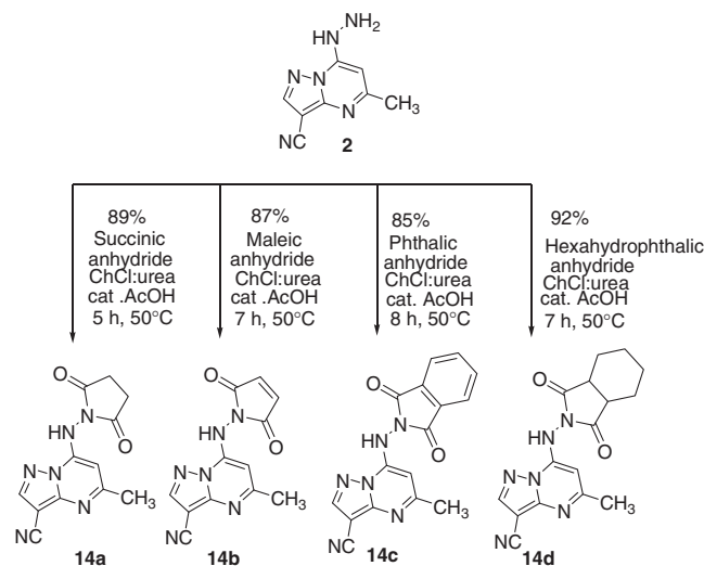
Scheme 5. Synthesis of dioxo pyrrolidones and dioxoisindol 14 a-d .
