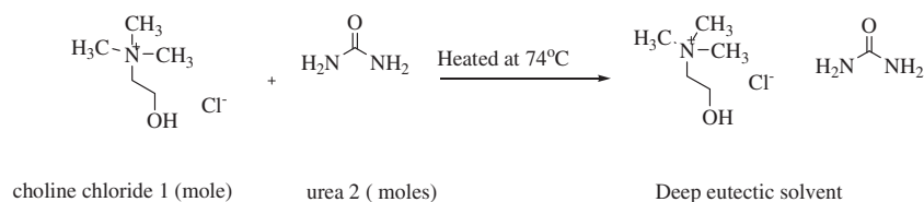
Figure 1. Preparation of deep eutectic mixture (DES).
