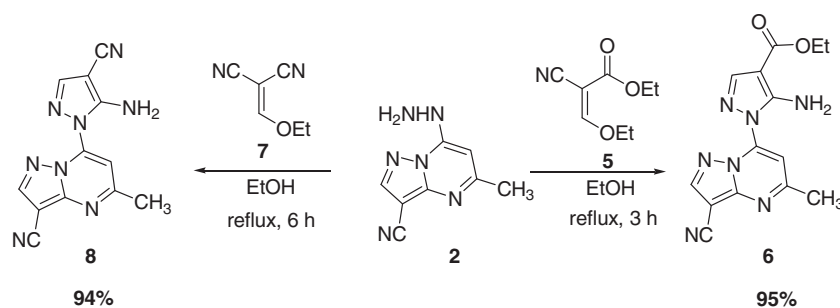
Scheme 2. Synthesis of Ethyl 5-amino-1-(3-cyano-5-methylpyrazolo[1,5- a ]pyrimidin-7-yl)-1 H -pyrazole-4-carboxylate 6 and 7-(5-Amino-4-cyano-1 H -pyrazol-1-yl)-5-methylpyrazolo[1,5- a ]pyrimidine-3-carbonitrile 8 .
