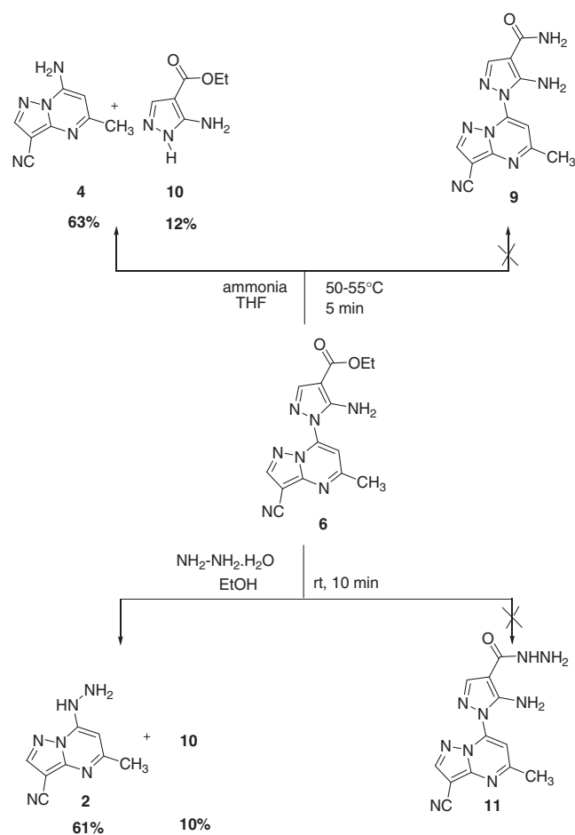
Scheme 3. Reaction on ethyl 5-amino-1-(3-cyano-5-methylpyrazolo[1,5- a ]pyrimidin-7-yl)-1 H -pyrazole-4-carboxylate.
