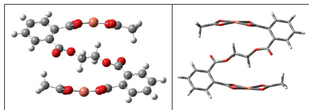
Figure 5. DFT optimized structures of (\text{CH}_3\text{COO})\text{Cu}(\text{II})\text{LCu}(\text{II})(\text{OOCCH}_3) . Pink = Cu(II); Red = O; Gray = C; White = H.
