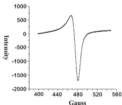
Figure 2. The X-band EPR spectra of (\text{CH}_3\text{COO})\text{Cu}(\text{II})\text{LCu}(\text{II})(\text{OOCCH}_3) recorded as the polycrystalline samples at room temperature.
