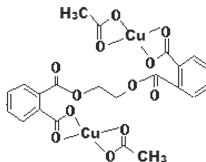
Scheme 2. Proposed structure of (\text{CH}_3\text{COO})\text{Cu}(\text{II})\text{LCu}(\text{II})(\text{OOCCH}_3) , confirmed by DFT calculation (figure 5).
