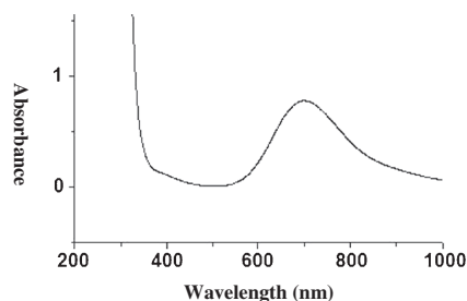
Figure 1. The UV/visible spectrum of (\text{CH}_3\text{COO})\text{Cu}(\text{II})\text{LCu}(\text{II})(\text{OOCCH}_3) in acetonitrile. ( 1 \times 10^{-3} M, path length 1.0 cm)
