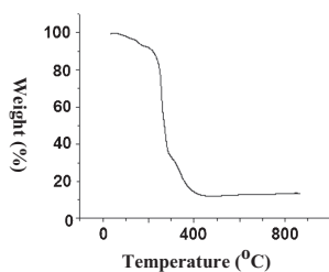
Figure 3. TGA curve of (\text{CH}_3\text{COO})\text{Cu}(\text{II})\text{LCu}(\text{II})(\text{OOCCH}_3) .
