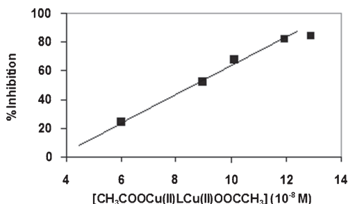
Figure 4. Plot of the percentage inhibition of superoxide formation against the (\text{CH}_3\text{COO})\text{Cu}(\text{II})\text{LCu}(\text{II})(\text{OOCCH}_3) concentration.
