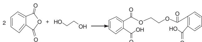
Scheme 1. Synthetic path for the ligand (L).
