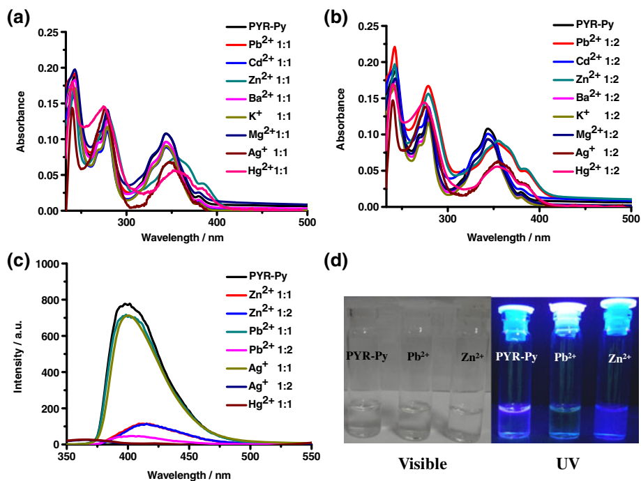
Figure 4. (a, b) UV-Vis spectra of PYR-Py, 10 -5 M in MeCN with various metal ions at 1:1 and 1:2 equivalents respectively, (c) PL spectra of PYR-Py, 10 -5 M in MeCN excited at 350 nm and (d) photograph showing visual changes to PYR-Py on addition of metal ions.
