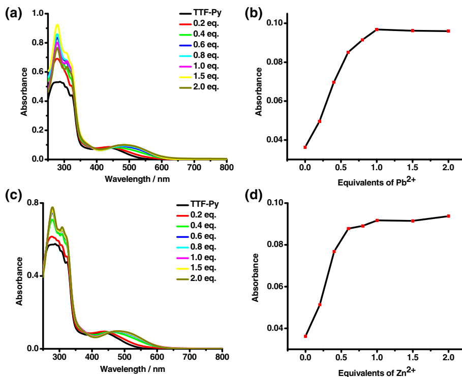
Figure 3. (a) UV-Vis spectra of various equivalents of Pb 2+ titrated with TTF-Py, (10 -4 M, in 1:1 CHCl 3 :MeCN), (b) plot of equivalents of Pb 2+ vs absorbance of the conjugate at 500 nm, (c) UV-Vis spectra of various equivalents of Zn 2+ titrated with TTF-Py, (10 -4 M, in 1:1 CHCl 3 :MeCN) and (d) plot of equivalents of Zn 2+ vs absorbance of the conjugate at 500 nm.
