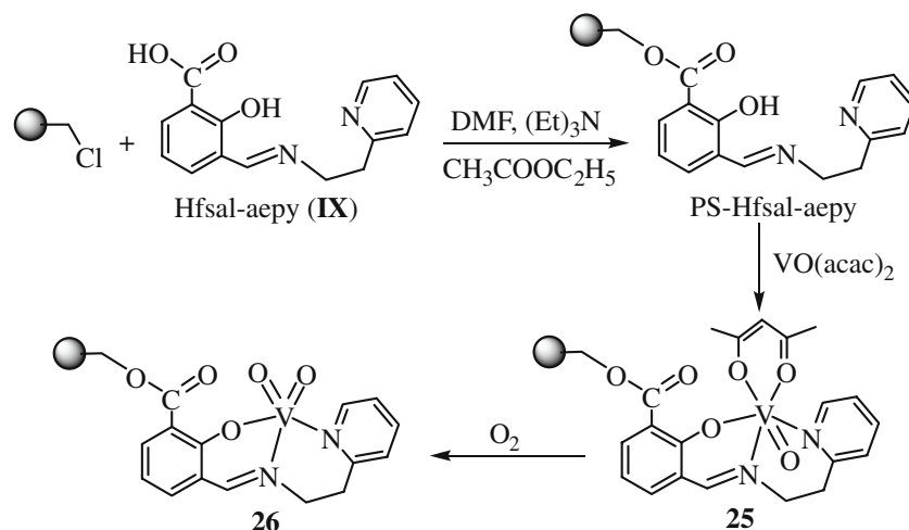
Scheme 9. Scheme for the synthesis of polymer-supported complexes. 29
