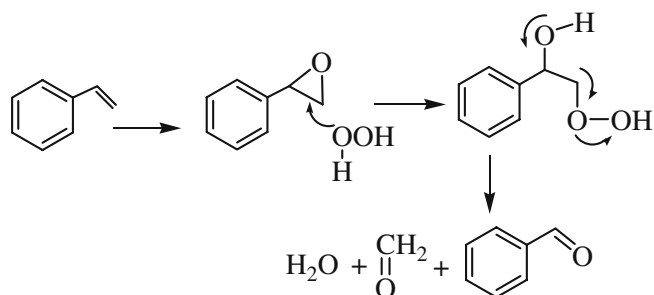
Scheme 15. Proposed mechanism.
