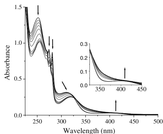
Figure 1. Titration of [\text{V}^{\text{V}}\text{O}_2(\text{sal-aebmz})] ( 4 ) with 30% \text{H}_2\text{O}_2 in MeOH. The spectra were recorded after successive addition of 1-drop portions of \text{H}_2\text{O}_2 dissolved in MeOH to 10 mL of a ca. 1 \times 10^{-4} M solution of 4 . 17
