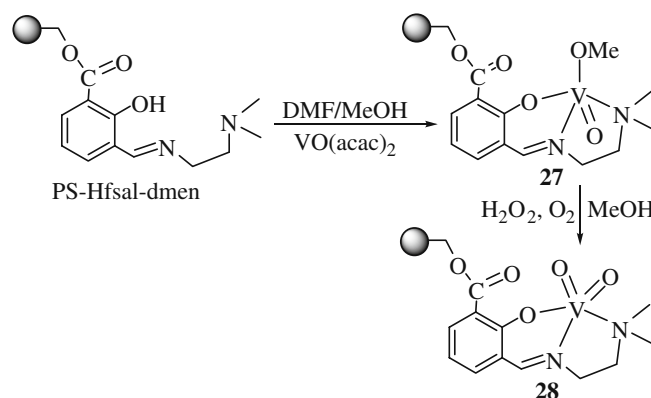
Scheme 10. Formation of PS-[V^{IV}O(OMe)(fsal-dmen)] ( 27 ) and PS-[V^VO_2(fsalsal-dmen)] ( 28 ). 30
