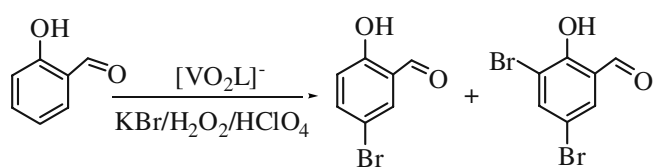
Scheme 11. Oxidative bromination of salicylaldehyde.
