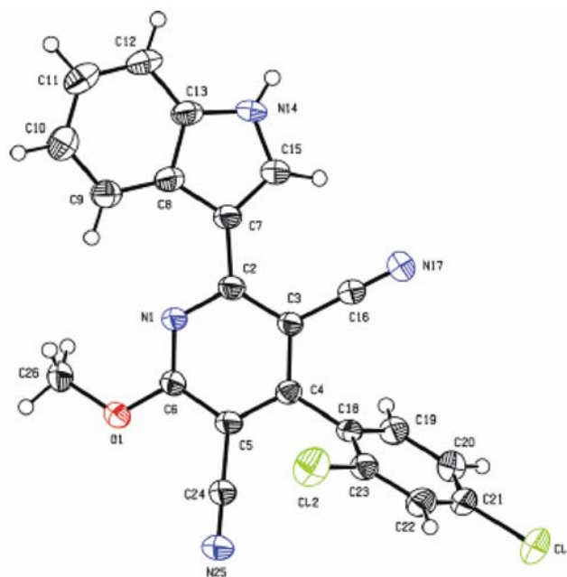
Figure 2. ORTEP diagram of compound 4g .
