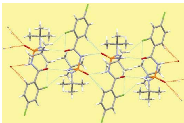
Figure 5. A one-dimensional polymeric chain produced by strong –P=O...H–N–, rather strong and weak C–H...O plus weak C–H...Cl hydrogen bonds in the crystalline lattice of compound 5 .
