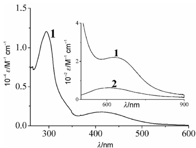
Figure 1. Electronic spectra of [\text{Cu}(\mu\text{-RSSR})_2 ( 1 ) in DMF-Tris buffer (1 : 1 v/v) medium. The inset shows the d-d band of the complexes 1 and 2 .
