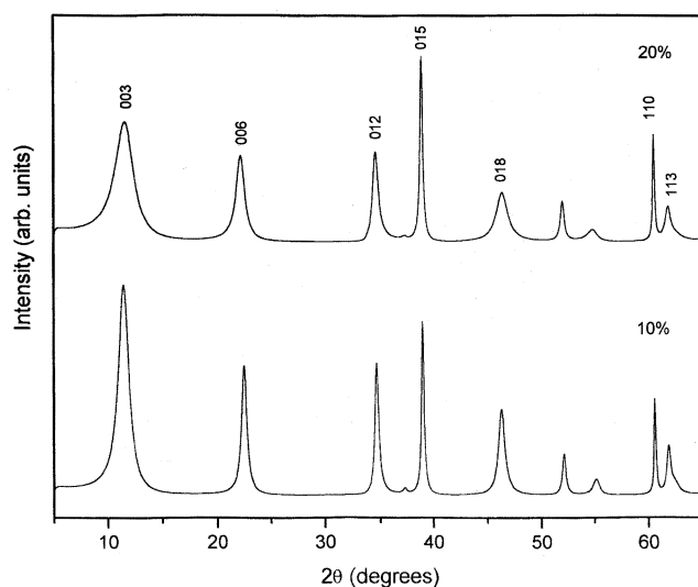
Figure 5. Simulated PXRD patterns of the \text{Mg-Fe-CO}_3^{2-} LDH interstratified with different percentages of \text{Mg}(\text{OH})_2 .
