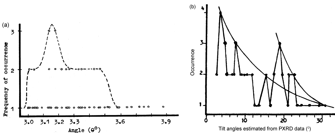
Figure 5. (a) Distribution of the value of angle \mathbf{q} , in case of different binary mixtures of C28 : C x ( x = 10, 12, 14, 16, 18 ). (b) Exponential nature of distribution angles.
