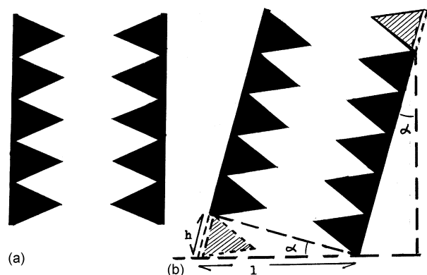
Figure 7. A schematic representation of vertical and tilted molecular chains: (a) saw teeth model; (b) relation between a and h .
