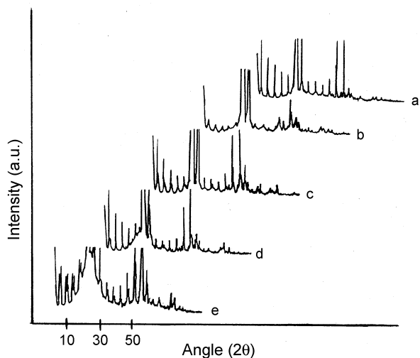
Figure 1. PXRD patterns of C28 : C10 binary mixtures; MR values: (a) 1.9067; (b) 1.5876; (c) 0.9962; (d) 0.6254; (e) 0.2746.
