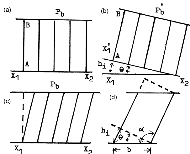
Figure 4. (a)–(c) Modifications of vertical structure to inclined structure. (d) Minimum displacement and related angle: b = 7.42 Å in b_m phase of C28.
