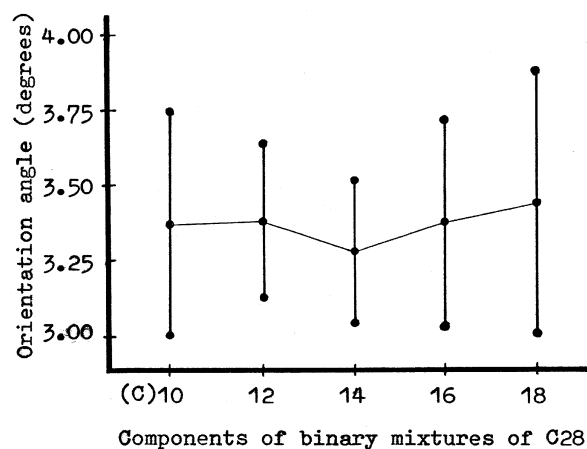
Figure 3. Extent of dispersion in the angle of orientation \mathbf{q} (of C28 molecule), in case of binary mixtures of C28 with different shorter chain hydrocarbons.
