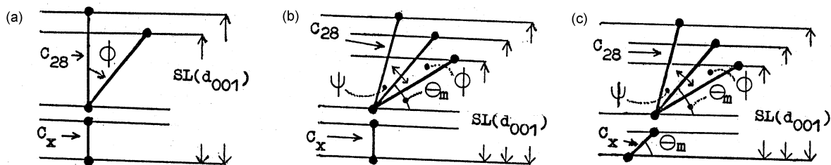
Figure 2. Superlattices in C28 : C x ( x = 10, 12, 14, 16 ) mixture systems. (a) b_0 - b_0 (C28 and C x are in the b_0 phase): Fluctuations in the orientation of C28 (from the vertical mode or b_0 phase) can lead to different b_0 - b_0 forms; (b) b_0 - b_m (C x in b_0 phase; C28 with different orientations in b_m phase). Clockwise rotation = angle f ; anti-clockwise rotation = angle y . (c) b_m - b_m (C x in b phase; C28 with different orientations in b_m phase).
