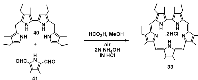
Scheme 10.
