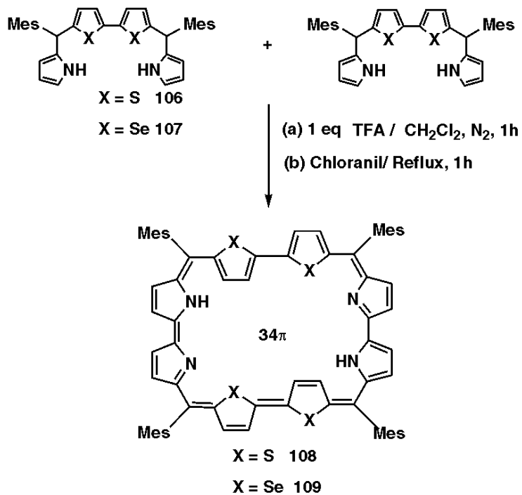
Scheme 35.
