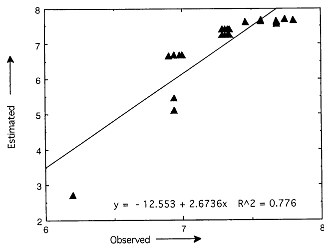
Figure 2. Correlation of observed and estimated \log pK_1^H of SHA derivatives used in the present study.
