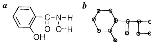
Figure 1. Molecular structure (a) and molecular graph (b) of SHA.
