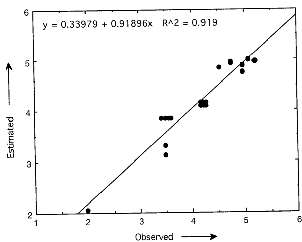
Figure 3. Correlation of observed and estimated \log pK_2^H of SHA derivatives used in the present study.
