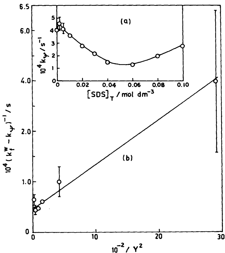
Figure 3. (a) k_{obs}/s^{-1} versus [SDS]_T/mol\ dm^{-3} plot at 35.0^\circ C ; [complex]_T = 3.6 \times 10^{-4} , [SO_3^{2-}]_T = 0.06 and [OH^-]_T = 0.10\ mol\ dm^{-3} . (b) (k_f^w - k_\psi)^{-1}(s) versus Y^{-2} plot.
