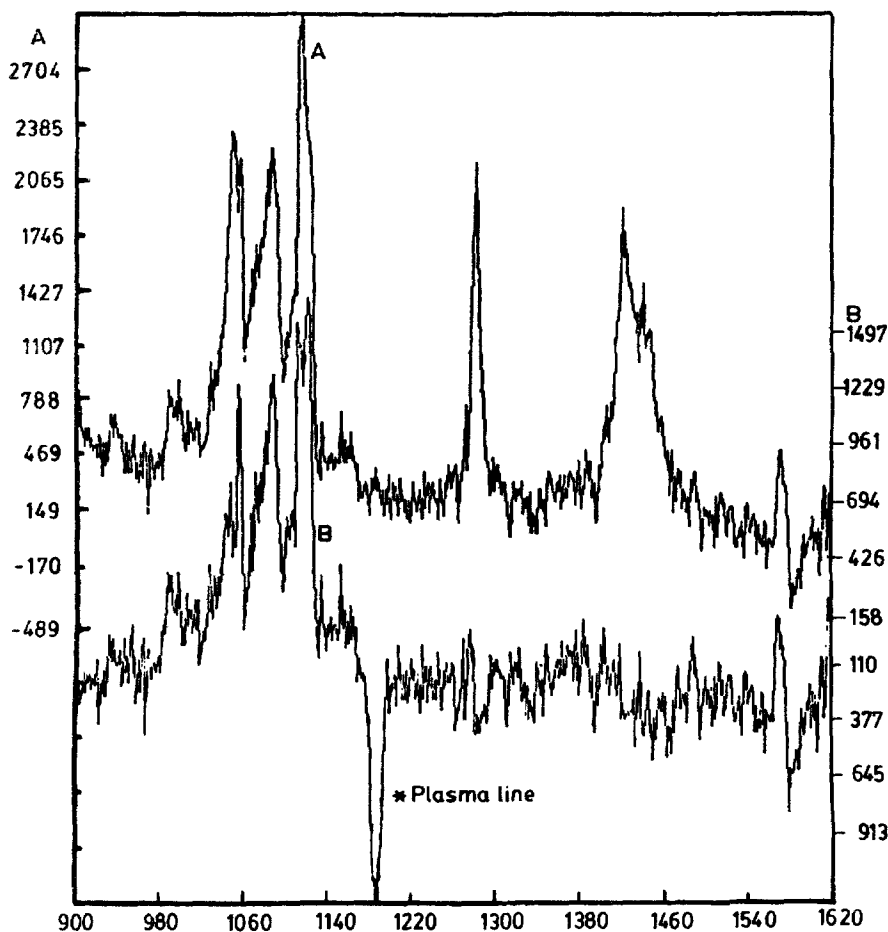
Figure 3. Difference spectra of (A) {DPPC + Dapsone}–Dapsone and (B) {DPPC + Dapsone}–DPPC–Dapsone in the region 900\text{--}1600\text{ cm}^{-1} .
