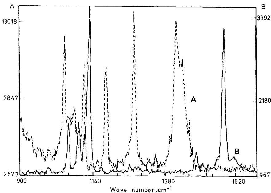
Figure 1. Laser Raman spectra of (A) Dapsone and (B) DPPC in the region 900–1700 \text{cm}^{-1} .
