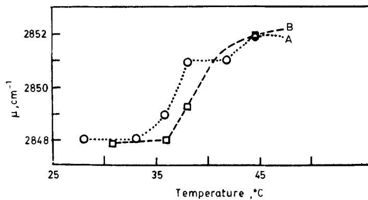
Figure 5. The premelting and melting transition of DPPC without (A) and with (B) Dapsone.
