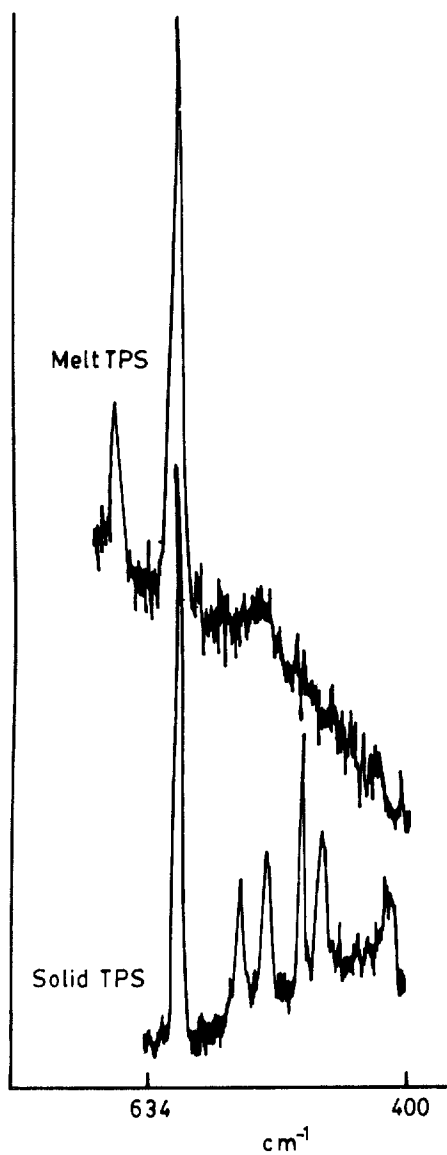
Figure 4. Raman spectra of TPS in solid and melt. The bands due to restricted rotation in solid are absent in the melt, only ring modes being left.
