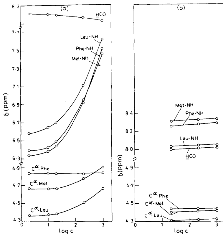
Figure 6. Concentration dependence of chemical shifts ( \delta ) for various resonances in Formyl-Met-Leu-Phe-OMe in \text{CDCl}_3 (a) and (\text{CD}_3)_2\text{SO} (b). Abscissa expresses concentration as \log c , where c = molar concentration of peptide \times 10^4 (from Raj and Balaram 1985).
