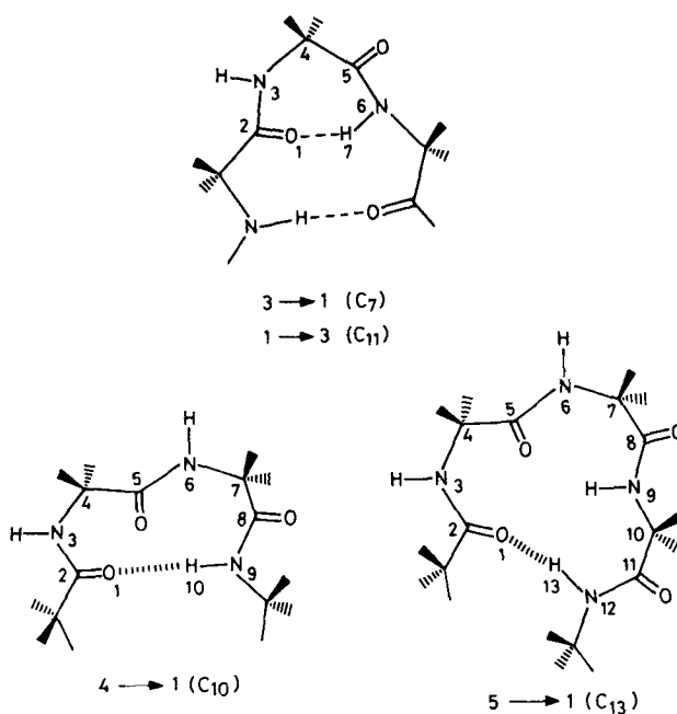
Figure 3. Representative intramolecularly hydrogen bonded conformations in peptides.
