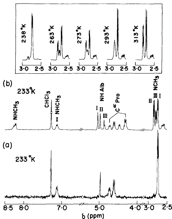
Figure 17. (a) Low temperature 270 MHz ^1\text{H} NMR spectrum of single crystals of Boc-Aib-Pro-Pro-NHMe recorded immediately after dissolution in \text{CDCl}_3 , pre-cooled in liquid \text{N}_2 and transferred to the probe at 233 K. (b) Low temperature 270 MHz ^1\text{H} NMR spectrum of a noncrystalline sample of Boc-Aib-Pro-Pro-NHMe at 233 K in \text{CDCl}_3 . (Inset) Methylamide \text{CH}_3 resonances (doublets) in Boc-Aib-Pro-Pro-NHMe. The sample was prepared as in (a) and the spectra recorded at various temperatures. I, II, III indicate an assignment to the Pro-Pro conformers described in figure 16 (from Balaram et al 1983).
