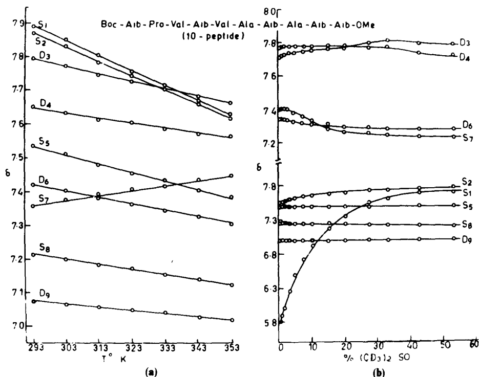
Figure 4. (a) Temperature dependence of NH chemical shifts in the decapeptide Boc-Aib-Pro-Val-Aib-Val-Ala-Aib-Ala-Aib-Aib-OMe in (\text{CD}_3)_2\text{SO} . S_n , D_n refer to singlet and doublet NH resonances. The subscript n refers to the order of appearance from low field in (\text{CD}_3)_2\text{SO} . (b) Dependence of NH chemical shifts on solvent composition in \text{CDCl}_3 - (\text{CD}_3)_2\text{SO} mixtures (from Iqbal and Balaram 1981a).
