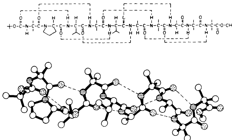
Figure 5. (bottom) Solid state conformation of Boc-Aib-Pro-Val-Aib-Val-Ala-Aib-Ala-Aib-Aib-OMe determined by x-ray diffraction (Francis et al 1983). Note 3_{10} -helical ( 4 \rightarrow 1 ) hydrogen bonding pattern. (top) Intramolecular hydrogen bonding scheme proposed on the basis of ^1\text{H} NMR studies (Iqbal and Balaram 1981a).
