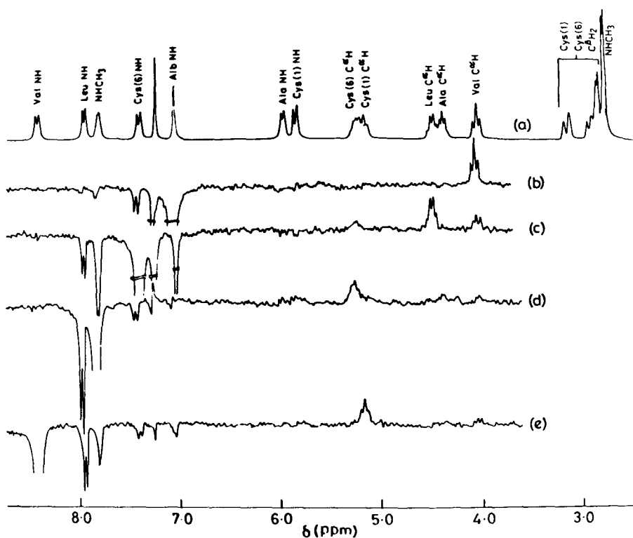
Figure 14. (a) Partial 270 MHz ^1\text{H} NMR spectrum of Boc-Cys-Val-Aib-Ala-Leu-Cys-
