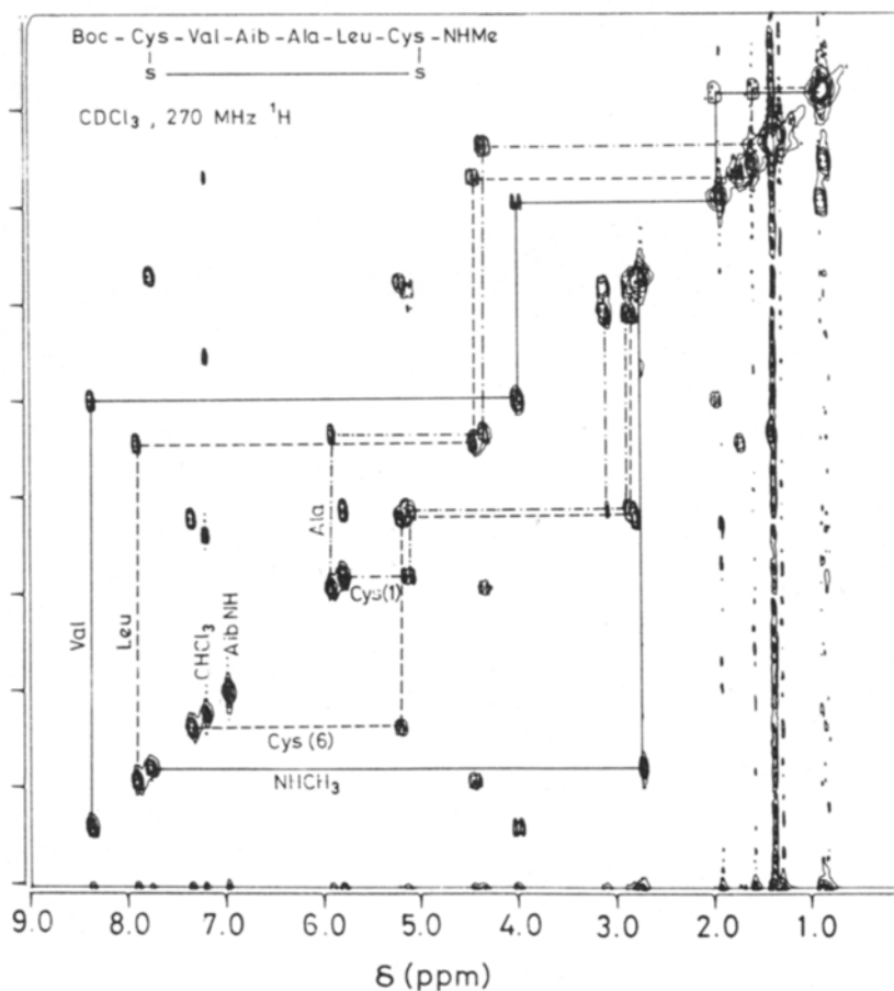
Figure 1. 270 MHz ^1\text{H} cosy spectrum (contour plot) of the peptide Boc-Cys-Val-Aib-Ala-Leu-Cys-NHMe in CDCl 3 . Connectivities of NH-C \alpha -H-C \beta H 2 protons
