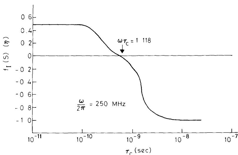
Figure 12. Dependence of ^1\text{H} - ^1\text{H} NOE magnitude ( \eta ) on the correlation time \tau_c (from Balaram et al 1973).
