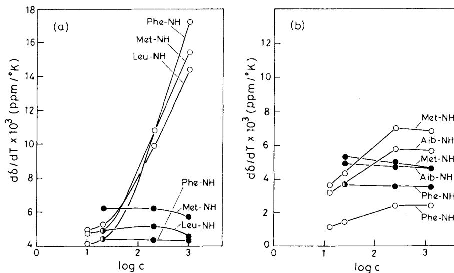
Figure 7. Concentration dependence of temperature coefficients ( d\delta/dT ) of NH resonances in chemotactic peptide analogs. (a) Formyl-Met-Leu-Phe-OMe ● (\text{CD}_3)_2\text{SO} ; ○ \text{CDCl}_3 (b) Formyl-Met-Aib-Phe-OMe ● (\text{CD}_3)_2\text{SO} ; ○ \text{CDCl}_3 -Abscissa defined as in figure 6 (from Raj and Balaram 1985).
