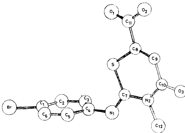
Figure 2. Crystal structure of 2-( p -bromophenyl-imino)-3,4-dihydro-3-methyl-4-oxo-2H-(1,3)-thiazine-6-carboxylic acid (7).
