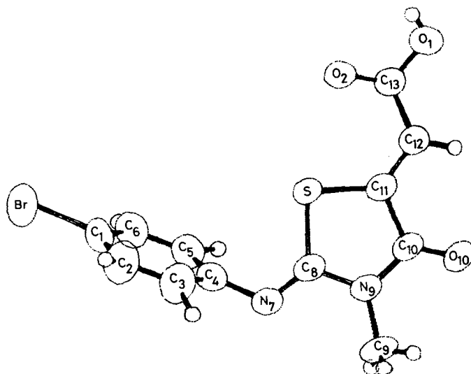
Figure 1. Crystal structure of 2-( p -bromophenyl-imino)-5-carboxymethylenethiazolidin-4-one (5).
