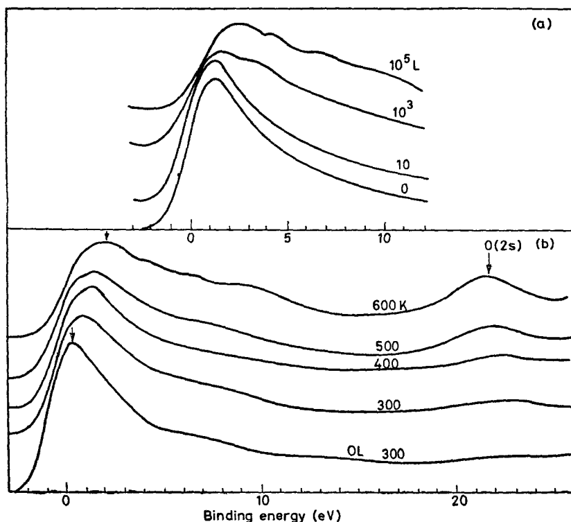
Figure 1. Valence band regions in the Al K_{\alpha} x-ray photoelectron spectra of clean cobalt and cobalt subjected to different oxygen exposures at different temperatures. (a) change in valence band as a function of oxygen exposure at 600 K; (b) temperature variation of valence band at 10 4 L exposure.
