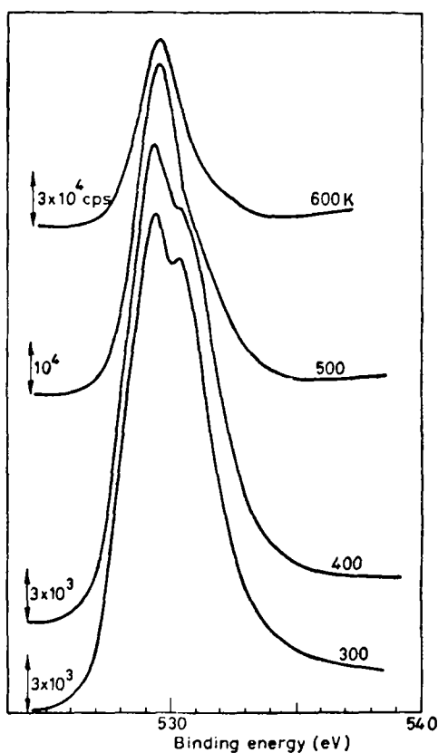
Figure 4. O(1s) band during the surface oxidation of Co (at 10^4 L) at different temperatures.
