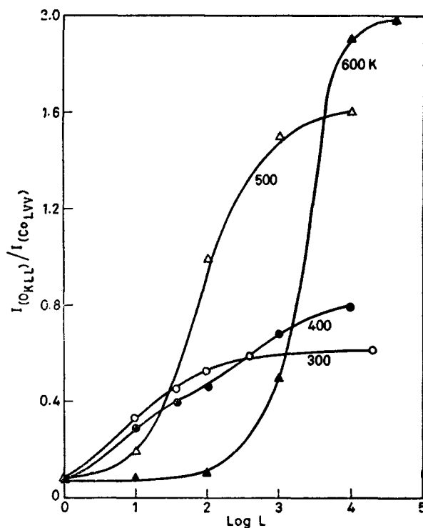
Figure 7. Plots of O (KLL)/Co ( L_{23}M_{45}M_{45} ) Auger intensity ratio against \log L at different temperatures.
