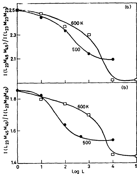
Figure 6. Plots of (a) L_{23}M_{45}M_{45}/L_{23}M_{23}M_{23} and, (b) L_{23}M_{45}M_{45}/L_{23}M_{23}M_{45} cobalt Auger intensity ratios against \log L at 500 and 600 K.
