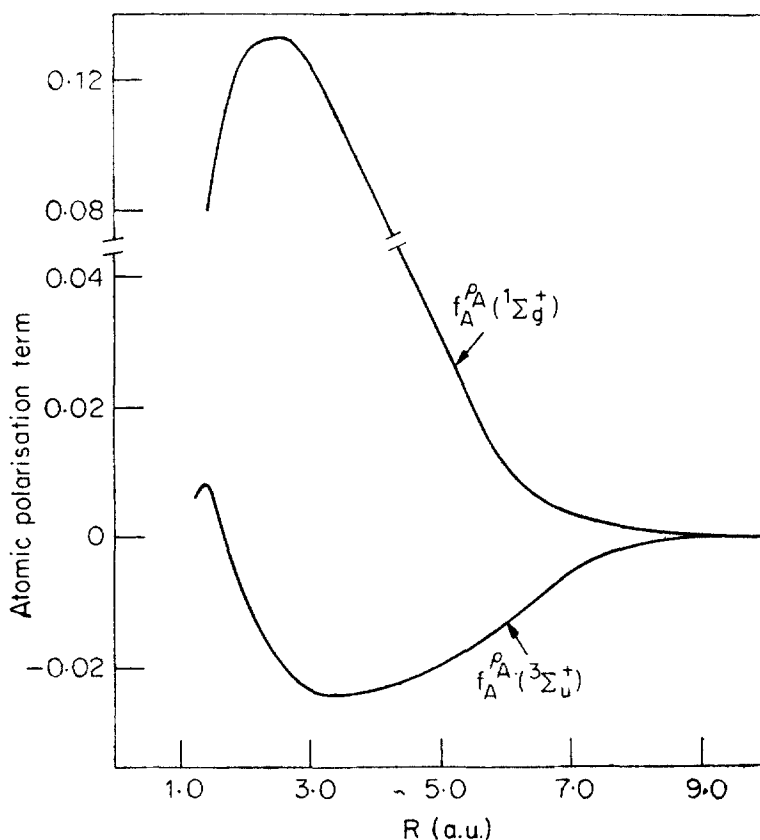
Figure 2. Variation with R of f_A^{\rho A} ( ^1\Sigma_g^+ ) and f_A^{\rho A} ( ^3\Sigma_u^+ ).
