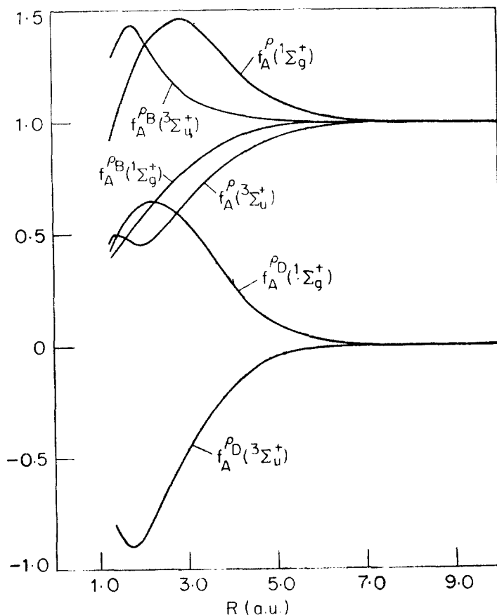
Figure 1. Variation with R of f_A^p(1\Sigma_g^+) , f_A^p(3\Sigma_u^+) , f_A^p(1\Sigma_g^+) , f_A^p(3\Sigma_u^+) , f_A^p(1\Sigma_g^+) and f_A^p(3\Sigma_u^+) . All the quantities are in atomic units.
