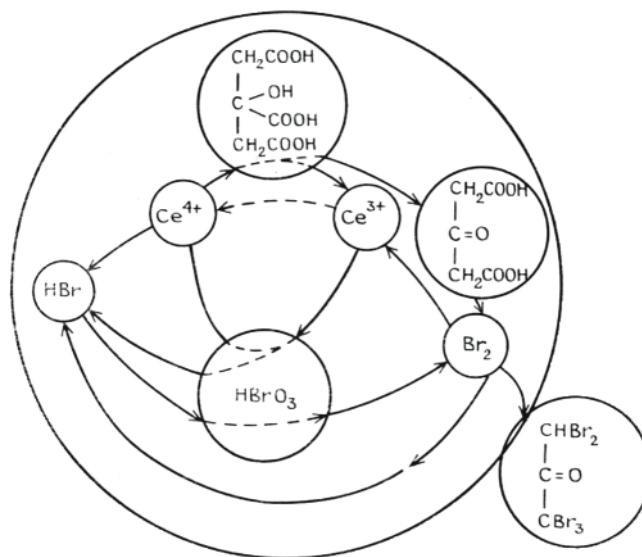
Figure 2. Belousov's scheme of his reaction.
