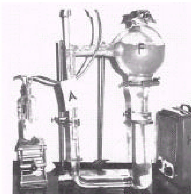
Figure 2. Apparatus for growing phage on a large scale. F, Fraser apparatus; H, electric fire; A, air line connected to sinter of F; T, air trap filled with cottonwool.
