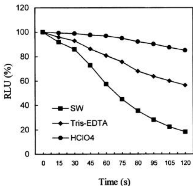
Figure 4. Effect of different extractants on the stability of luminescence signal. RLU, Relative light unit.
