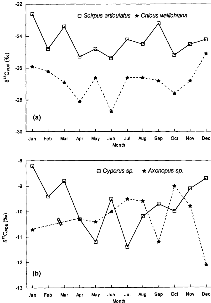
Figure 1. Monthly variations during 1995 in \delta^{13}\text{C}_{\text{PDB}} values of (a) C3 plants and (b) C4 plants growing in a peat bog at Sandynallah, southern India. Uncertainty ( 1\sigma = \pm 0.1\text{‰} ).
