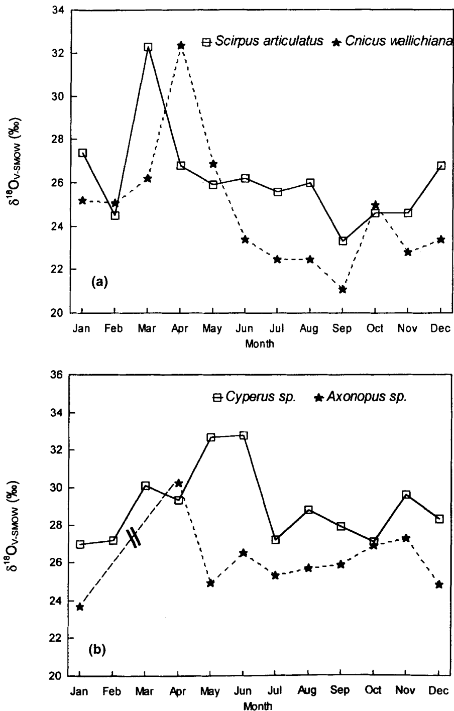
Figure 2. Monthly variations during 1995 in \delta^{18}\text{O}_{\text{SMOW}} values of (a) C3 plants and (b) C4 plants growing in a peat bog at Sandynallah, southern India. Uncertainty ( 1\sigma = \pm 0.25\text{‰} ).
