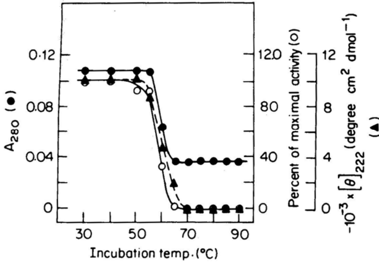
Figure 4. Effect of preincubation temperature on the structure ( A_{280} and -[\theta]_{222} ) and enzyme activity. The enzyme (270 \mu\text{g/ml} ) was heated at different temperatures (30°-90°C) for 10 min and immediately chilled in ice. The sample was used to measure the -[\theta]_{222} value ( \Delta ), A_{280} (O) at 25°C and enzyme activity at 37°C (O). Activity of the unheated enzyme was normalized to 100.
