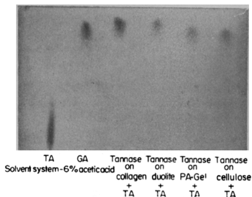
Figure 5. Paper chromatography of tannic acid and its hydrolyzed product by the action of immobilized tannase with standard gallic acid.
