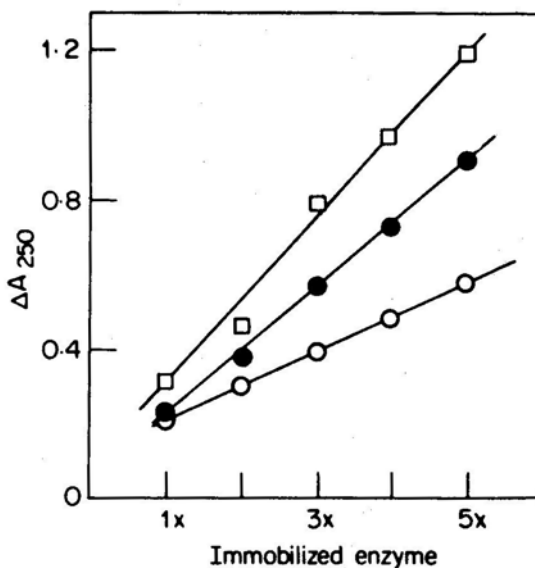
Figure 4. Effect of immobilized tannase at different concentrations. Collagen-enzyme (5 to 25 mg, \square ), Duolite-enzyme (20 to 100 mg, \circ ) and polacrylamide gel enzyme (50 to 250 mg, \bullet ), Ten ml of 0.008% tannic acid in 50 mM sodium acetate buffer (pH 4.7) was added. Incubation for 20 min at 25°C.
