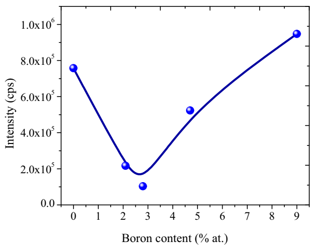
Figure 9. PL intensity vs. boron content.
