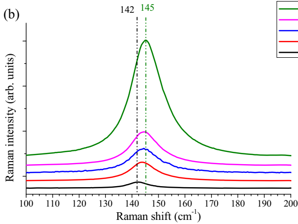
Figure 6. (a) Raman spectra of the B-modified TiO 2 thin films, (b) zoom of the 144 cm -1 Raman band.
