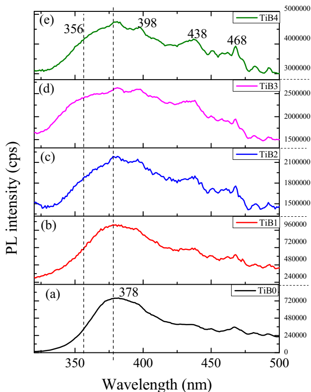
Figure 8. PL spectra of the different photocatalysts.
