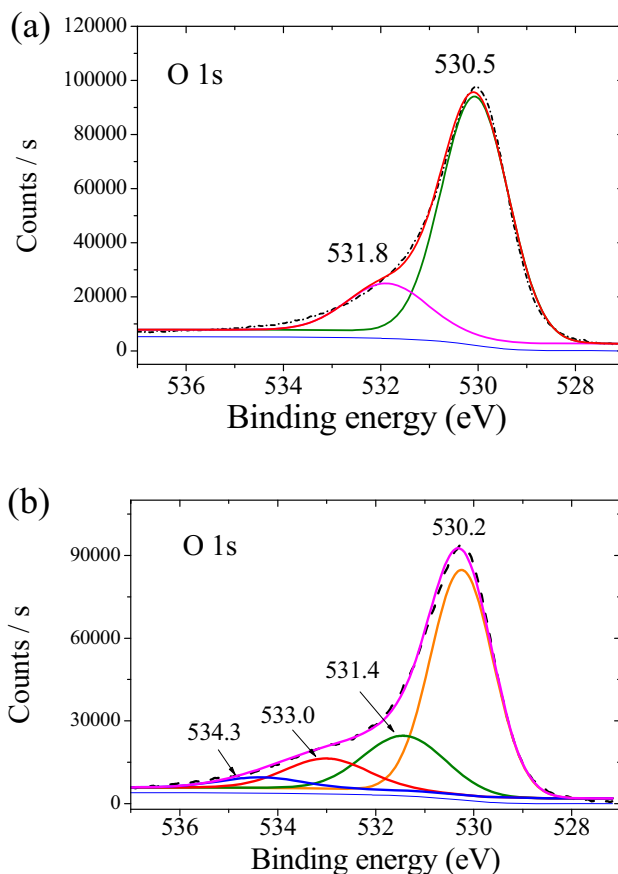
Figure 4. XPS O-1s region corresponding to films (a) without boron and (b) containing 9.0 at% of boron.
