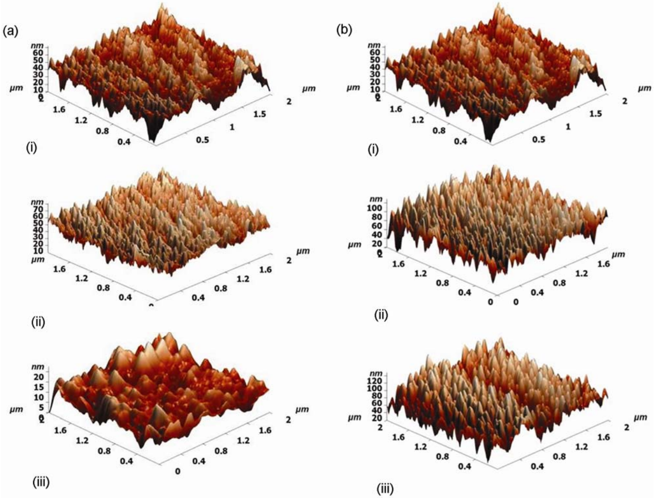
Figure 4. AFM surface morphologies of CrN thin films: (a) as a function of working pressure deposited at 200°C: (i) 10 mTorr, (ii) 15 mTorr and (iii) 20 mTorr and (b) as a function of temperature deposited at 10 mTorr pressure: (i) 200°C, (ii) 300°C and (iii) 400°C.
