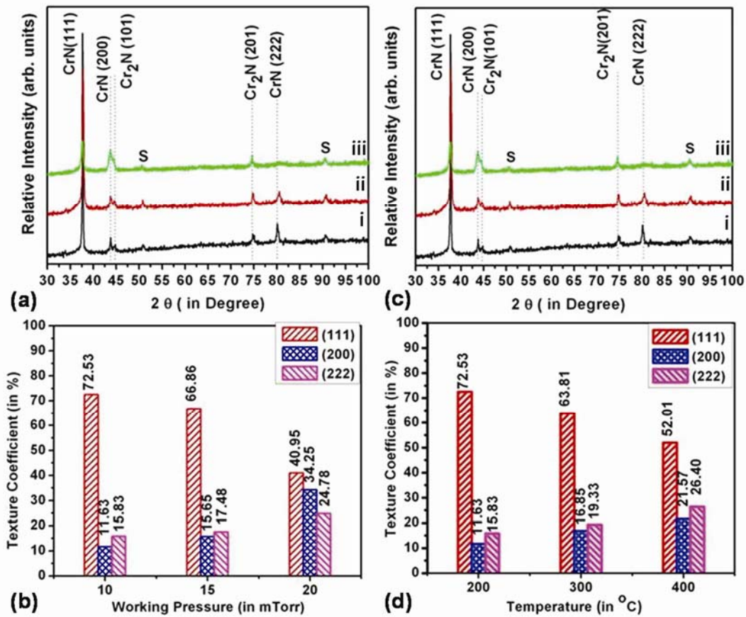
Figure 1. XRD peaks and texture coefficient of CrN films deposited on SS-304 substrate: (a) and (b) as a function of working pressure: (i) 10 mTorr, (ii) 15 mTorr, (iii) 20 mTorr, deposited at 200°C, while (c) and (d) as a function of temperature: (i) 200°C, (ii) 300°C and (iii) 400°C deposited at 10 mTorr.
