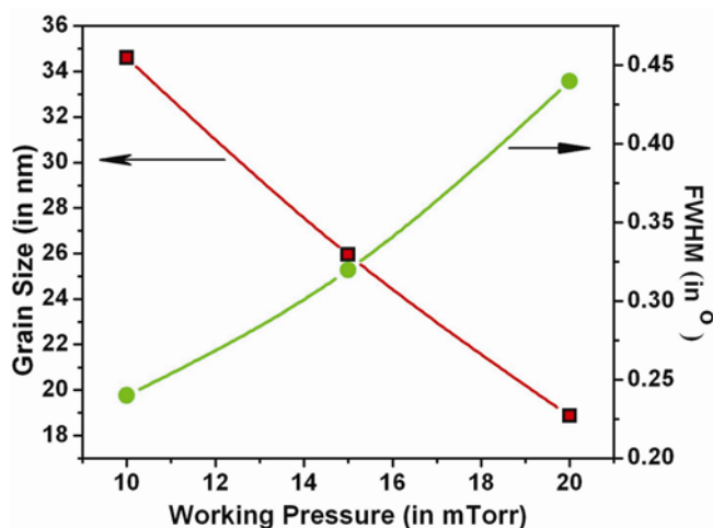
Figure 2. The dependence of the grain size and FWHM on the working pressure of CrN films deposited at 200°C and power, 75 W.
