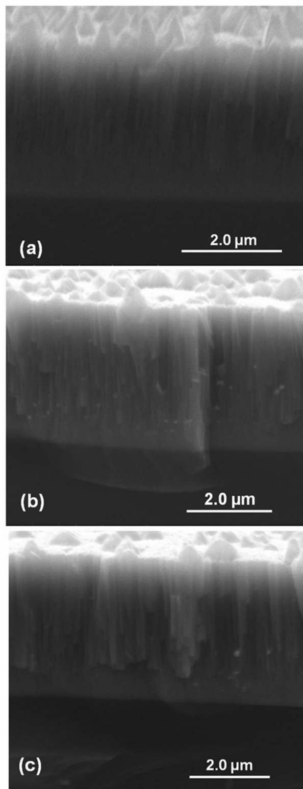
Figure 3. Scanning electron micrographs of fracture cross sections of CrN thin films deposited at different working pressure and temperature.
