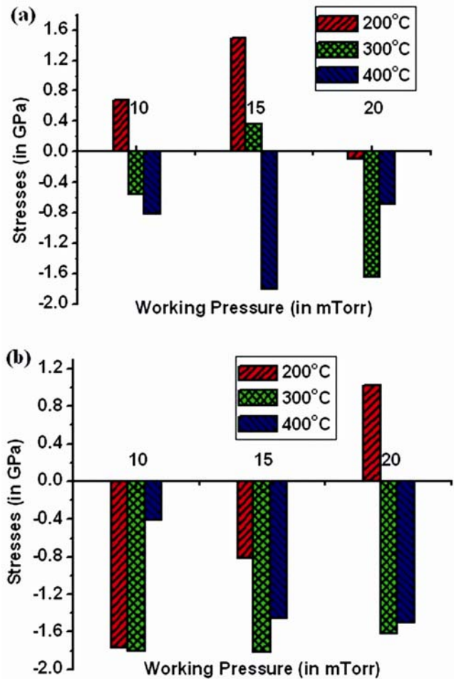
Figure 5. Intrinsic stresses produced in CrN films deposited at (a) 75 W and (b) 100 W.
