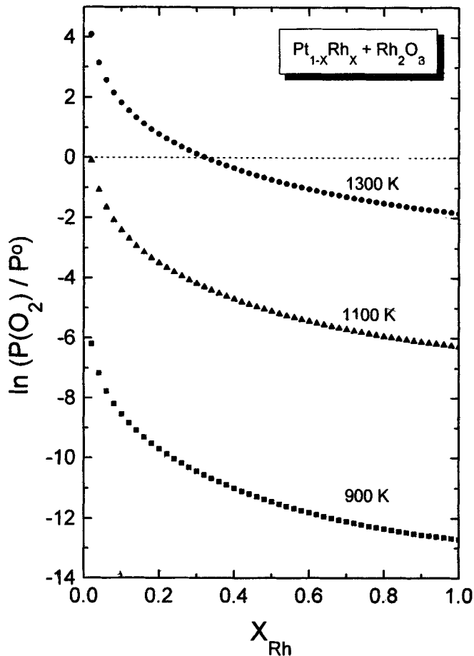
Figure 2. Variation of the equilibrium oxygen chemical potential for the formation of \text{Rh}_2\text{O}_3 as a function of composition of Pt-Rh alloys at different temperatures.
