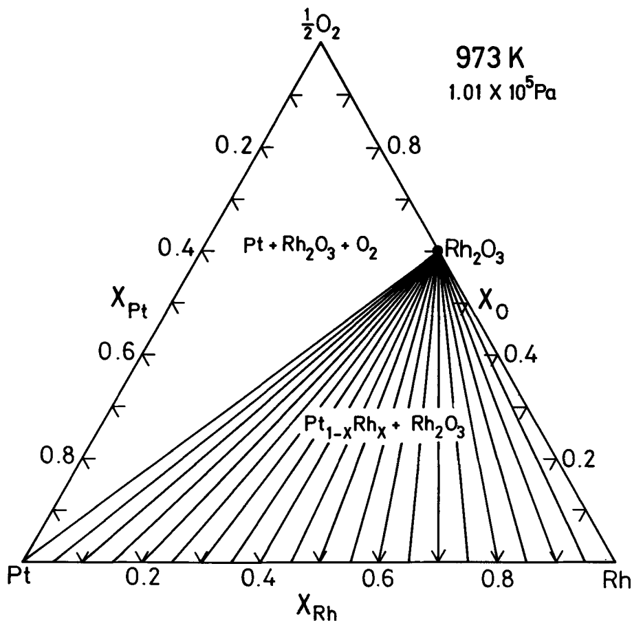
Figure 4. Isothermal section of the Pt-Rh-O system at 973 K computed from thermodynamic data.
