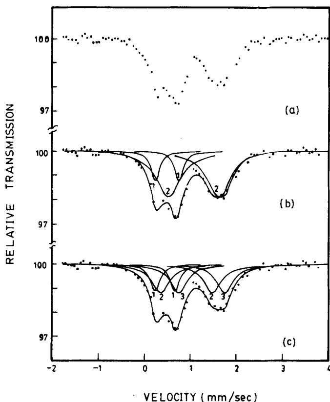
Figure 1. Mössbauer spectra of the sample C 1 at room temperature: (a) raw data, (b) 'two doublet' fit and (c) 'three doublet' fit.
