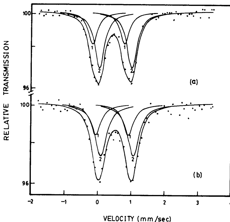
Figure 3. Mössbauer spectra of the sample C_2 : (a) at room temperature and (b) at 125 K.
