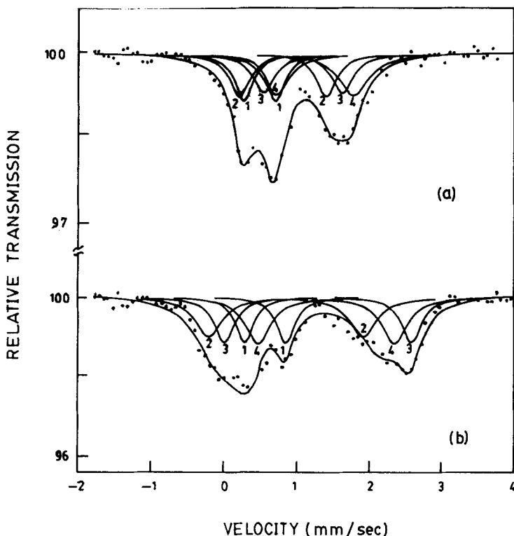
Figure 2. Mössbauer spectra of the sample C_1 with 'four doublet' fit: (a) at room temperature and (b) at 125 K.
