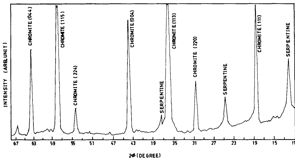
Figure 4. X-ray diffractogram of the sample C_1 .
