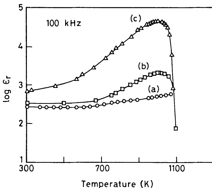
Figure 4. Variation of dielectric constants with temperature at 100 kHz for (a) \text{Bi}_2\text{WO}_6 , (b) \text{Bi}_2\text{O}_3-0.7\text{WO}_3-0.3\text{CuO} , and (c) \text{Bi}_2\text{O}_3-0.3\text{WO}_3-0.7\text{CuO} .
