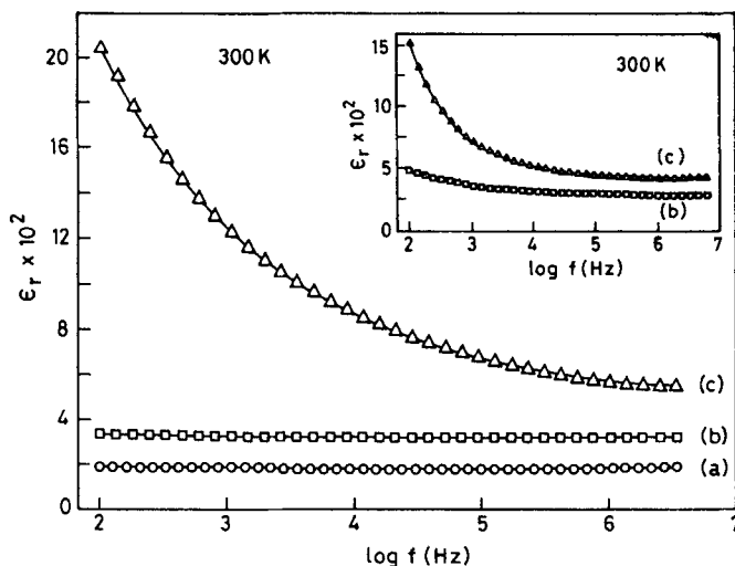
Figure 3. Frequency dependence of dielectric constant data at 300 K for (a) \text{Bi}_2\text{WO}_6 , (b) \text{Bi}_2\text{O}_3-0.7\text{WO}_3-0.3\text{CuO} , and (c) \text{Bi}_2\text{O}_3-0.3\text{WO}_3-0.7\text{CuO} . The inset shows the data for (b) and (c) with platinum electrodes.
