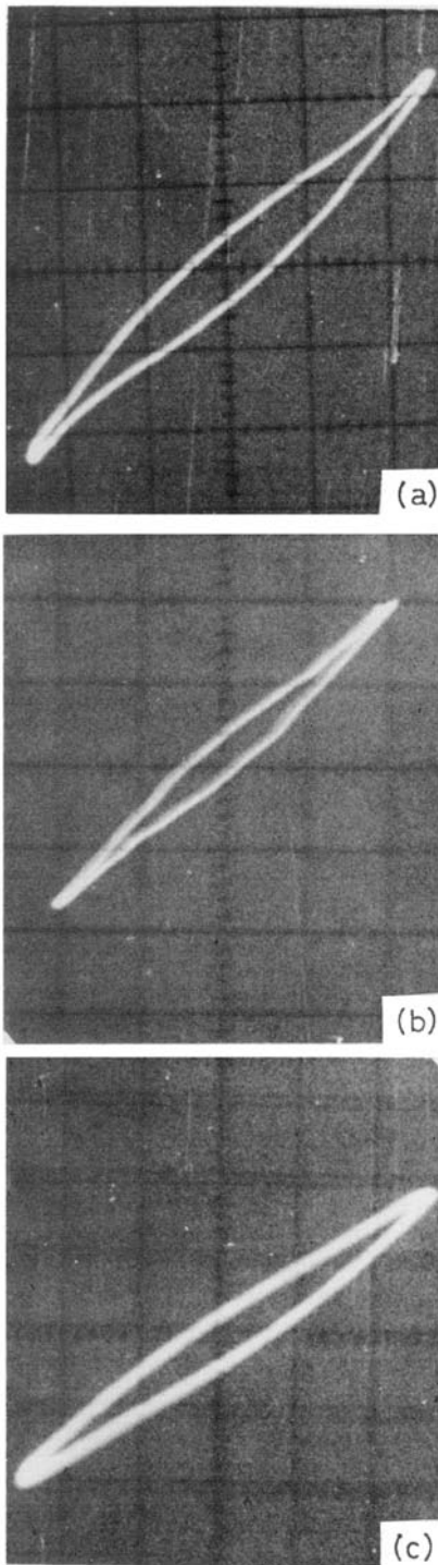
Figure 5. Ferroelectric hysteresis-loops for (a) \text{Bi}_2\text{WO}_6 , (b) \text{Bi}_2\text{O}_3-0.7\text{WO}_3-0.3\text{CuO} , and (c) \text{Bi}_2\text{O}_3-0.3\text{WO}_3-0.7\text{CuO} recorded at 300 K.
