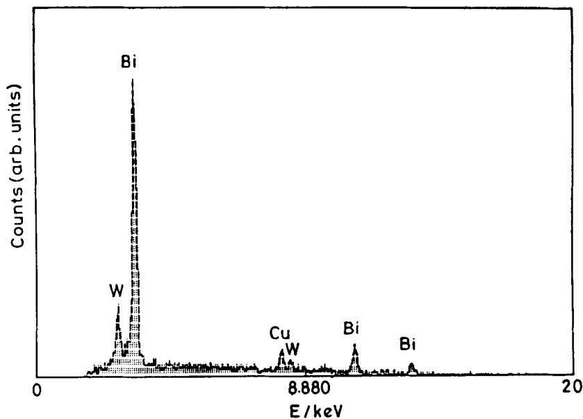
Figure 2. Compositional profile of \text{Bi}_2\text{O}_3-0.3\text{WO}_3-0.7\text{CuO} as obtained by EDAX.
