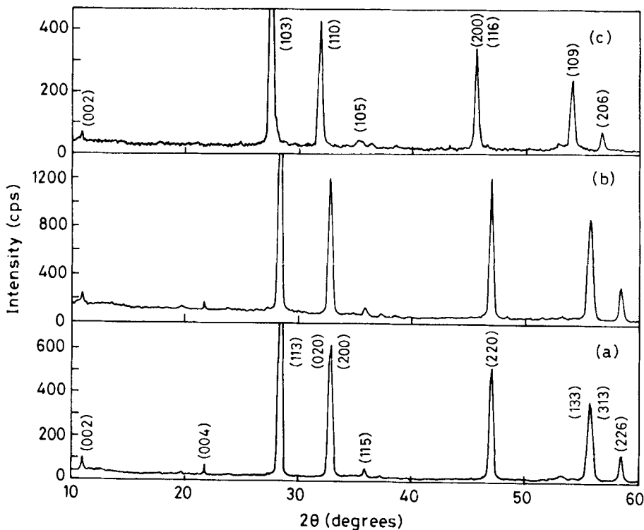
Figure 1. X-ray powder diffraction patterns for (a) \text{Bi}_2\text{WO}_6 , (b) \text{Bi}_2\text{O}_3-0.7\text{WO}_3-0.3\text{CuO} , and (c) \text{Bi}_2\text{O}_3-0.3\text{WO}_3-0.7\text{CuO} .
