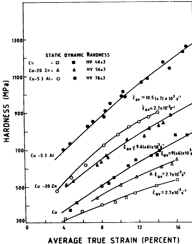
Figure 3. Variation of static and dynamic hardness as a function of average true strain for Cu, Cu-20% Zn and Cu-5.3% Al alloys.
