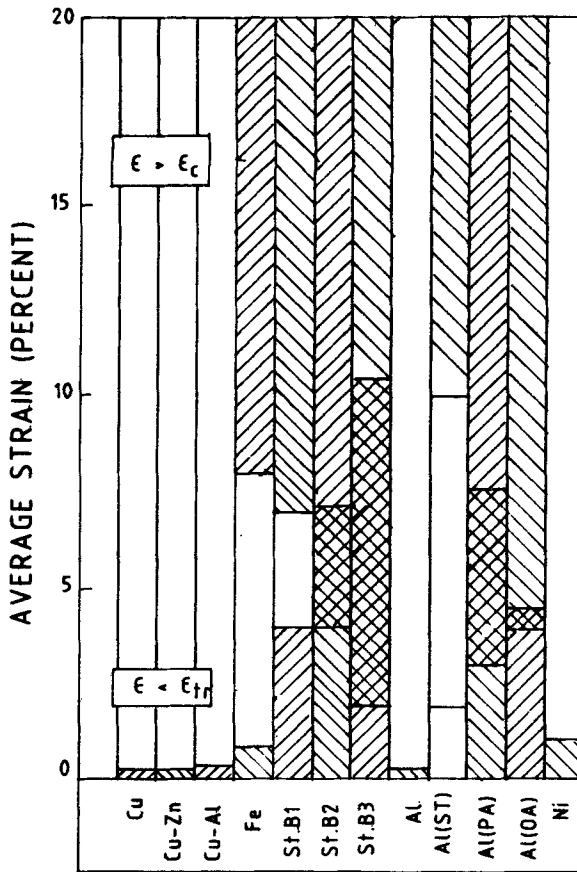
Figure 23. The computed values of \epsilon_{tr} (9) and the experimental values for \epsilon_c for a number of metals and alloys. Each bar in the figure represents one material.
