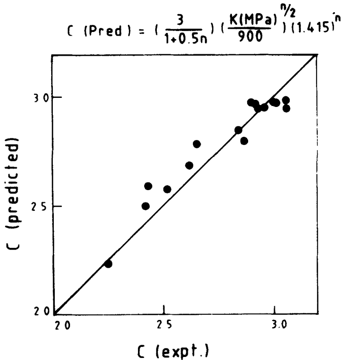
Figure 19. A comparison of the experimental value of C (table 1) with the value of C predicted by the empirical equations ((18) and (19) in the text) in the case of a number of metallic materials.
