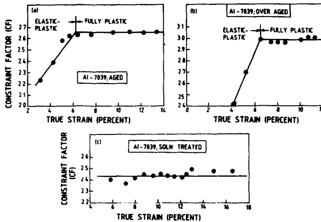
Figure 16. The variation of constraint factor of an Al 7039 alloy with true strain: (a) aged, (b) overaged and (c) solution treated.
