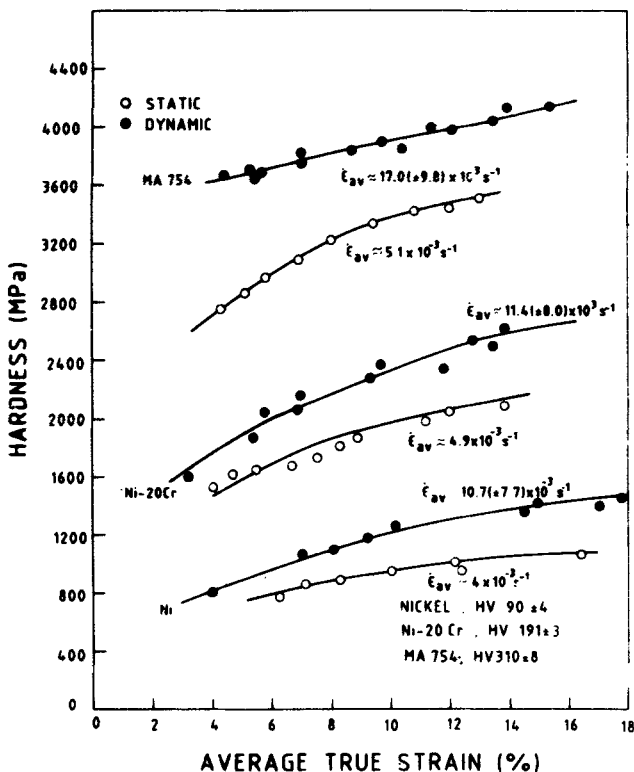
Figure 5. Variation of static and dynamic hardness as a function of average true strain for Ni, Ni-20% Cr and MA 754 alloy.
