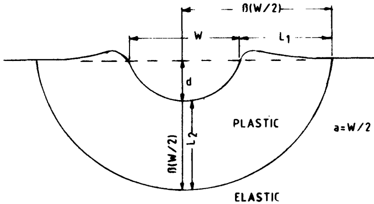
Figure 8. A schematic diagram of the plastic zone with the various parameters defined.
