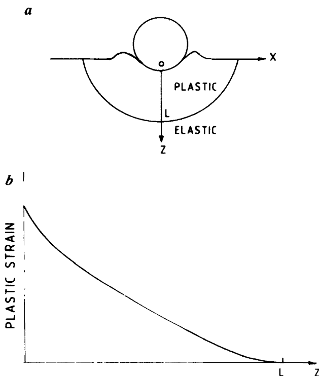
Figure 2. A schematic diagram illustrating the plastic zone formed beneath the indentation (a) and the plastic strain gradient within the plastic zone (b).
