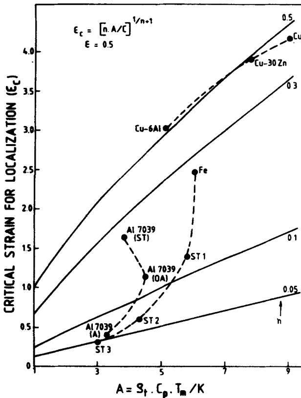
Figure 22. The variation of \epsilon_c predicted by (20) as a function of parameter A for a number of test materials.
