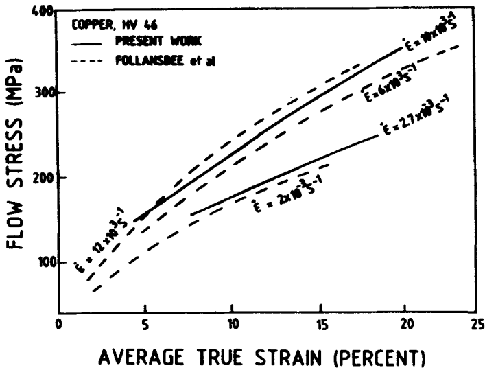
Figure 21. A comparison of the present dynamic and static data (full lines) for copper with that of Follansbee et al (dotted lines).
