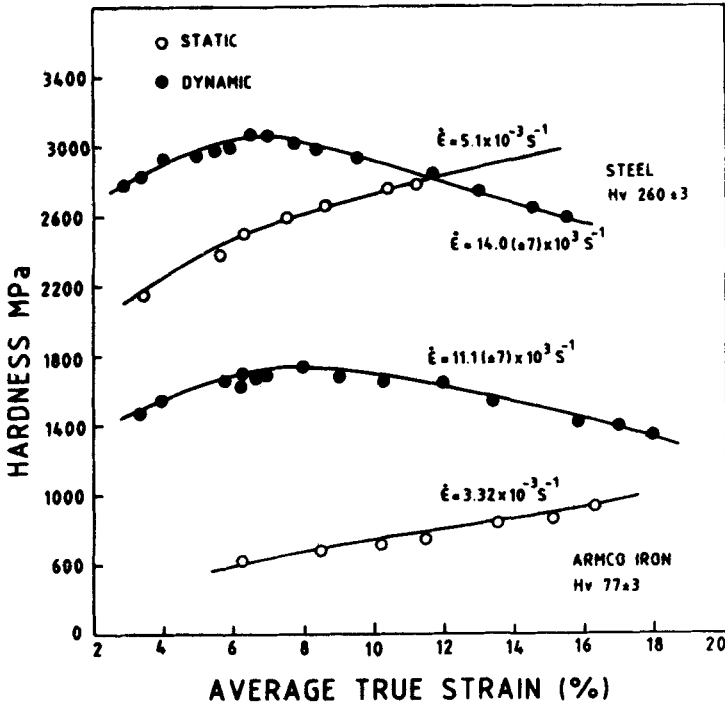
Figure 4. Variation of static and dynamic hardness as a function of average true strain for iron and steel B1 (Hv 260).
