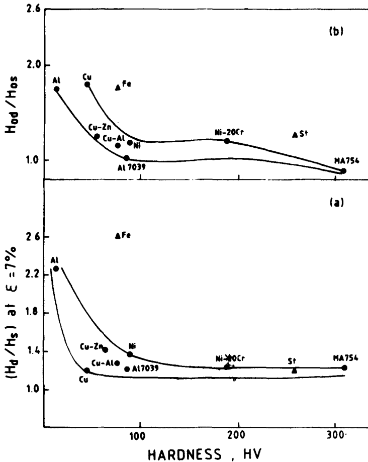
Figure 6. (a) The ratio of dynamic to static hardness ( H_d/H_s ) at a constant strain of 7% for a number of metallic materials and (b) the ratio H_{0d}/H_{0s} (defined by (8) and (9) in the text) for a number of metallic materials.
