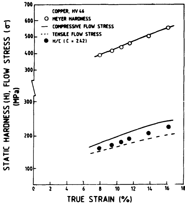
Figure 12. The experimental H_s - \epsilon_{av} and \sigma - \epsilon curves for copper. The filled circles represent the \sigma - \epsilon data derived from H_s - \epsilon_{av} curve.
