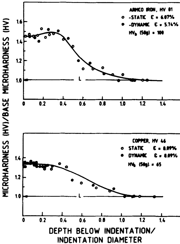
Figure 20. The microhardness–depth profiles obtained on statically and dynamically indented samples of iron and copper. In each of these profiles, the filled and unfilled symbols represent microhardness data obtained on dynamically and statically indented samples to nearly the same average strain.
