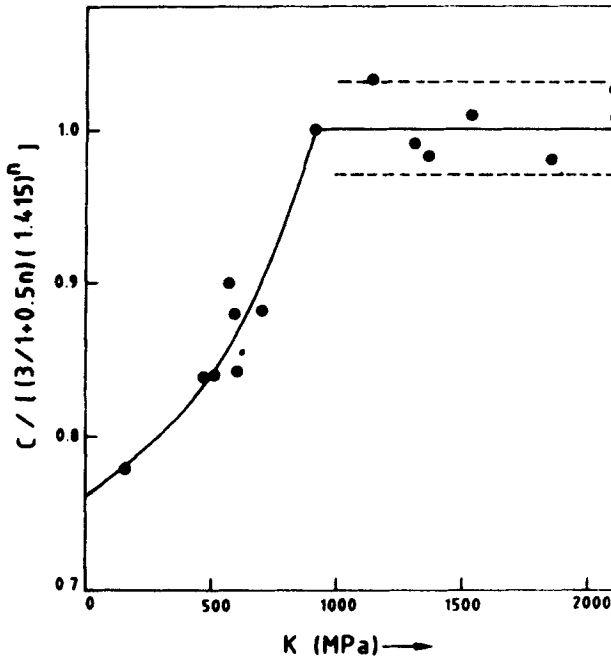
Figure 18. The variation of the ratio of experimental value of C (table 1) to the predicted value of C (17) with the strength coefficient ( K ).
