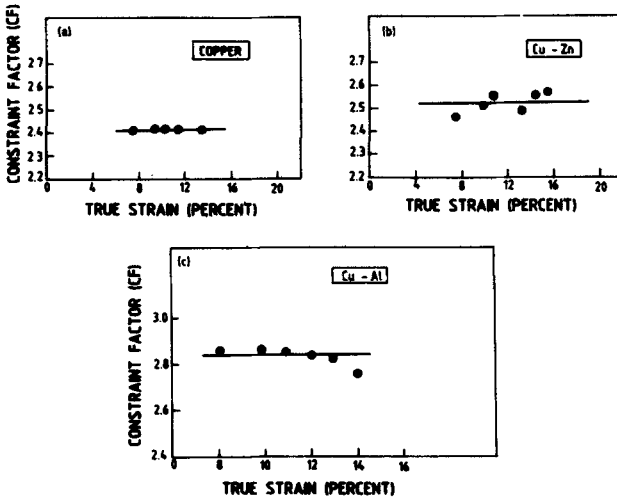
Figure 14. The variation of constraint factor with average true strain: (a) copper, (b) Cu-Zn alloy and (c) Cu- Al alloy.
