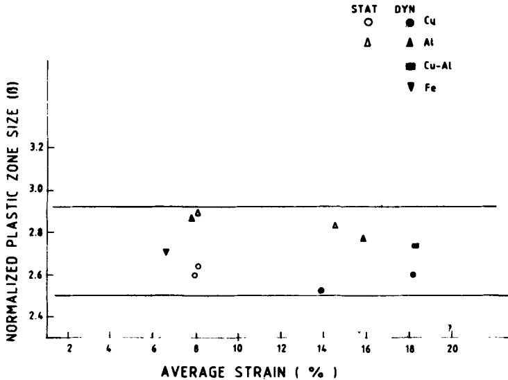
Figure 9. The variation of the normalized plastic zone size ( \beta ) with average strain ( \epsilon_{av} ) for a number of materials. The filled and unfilled symbols represent dynamic and static indentation data respectively.
