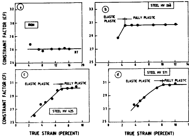
Figure 15. The variation of constraint factor with true strain: (a) iron, (b) steel, Hv 260; (c) steel, Hv 425; and (d) steel, Hv 571.
