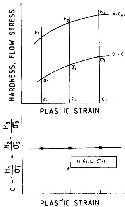
Figure 11. A schematic diagram illustrating the relationship between the H-\epsilon_{av} and the \sigma-\epsilon curves through the constraint factor ( C ).
