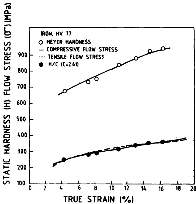
Figure 13. The experimental H_s - \epsilon_{av} and \sigma - \epsilon curves for iron. The filled circles represent the \sigma - \epsilon data derived from H_s - \epsilon_{av} curve.
