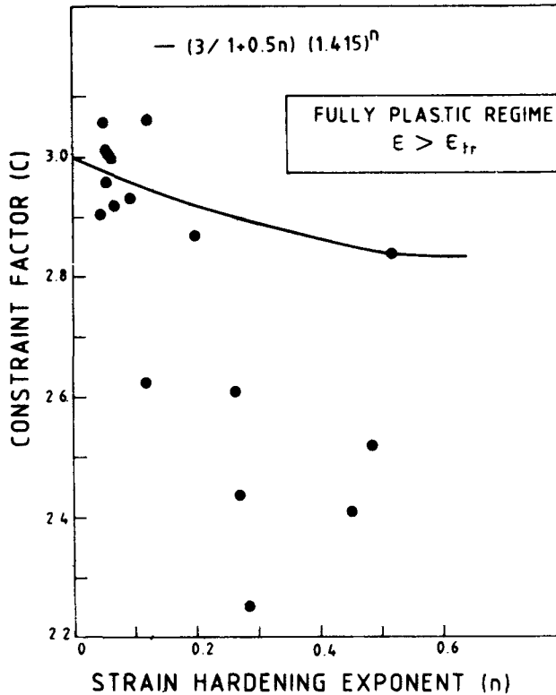
Figure 17. The variation of constraint factor ( C ) with strain hardening exponent ( n ). The value of C predicted by Mathews ((17) in the text) is represented by the full line.
