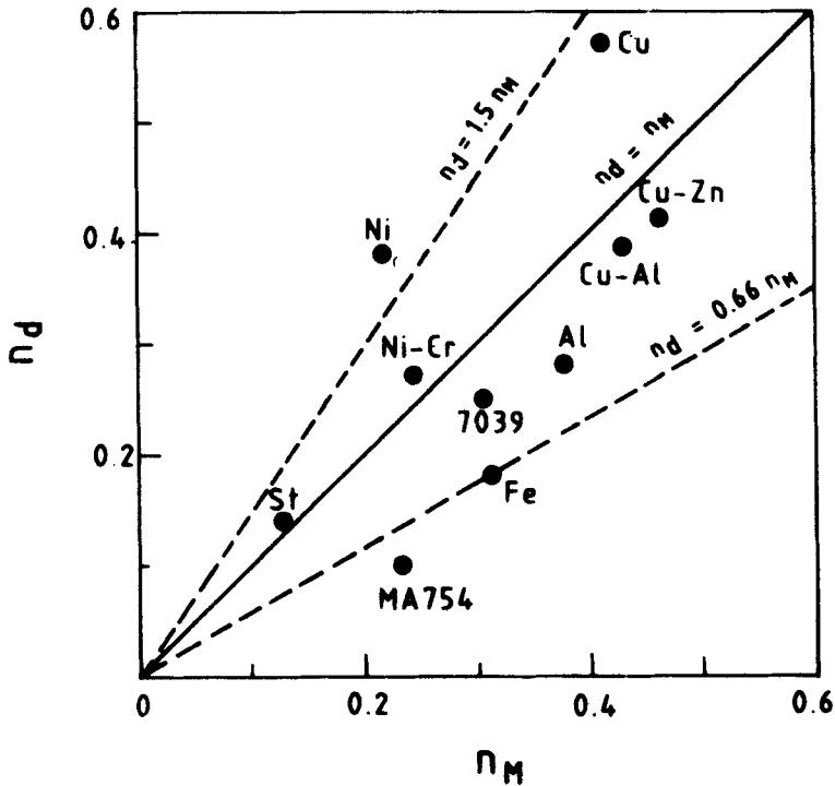
Figure 7. A comparison of static and dynamic strain hardening exponents ( n_M and n_D respectively) for a number of metals and alloys.
