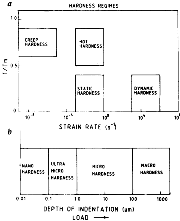
Figure 1. The classification of hardness tests on the basis of indentation test conditions (a) and depth of indentation (b).
