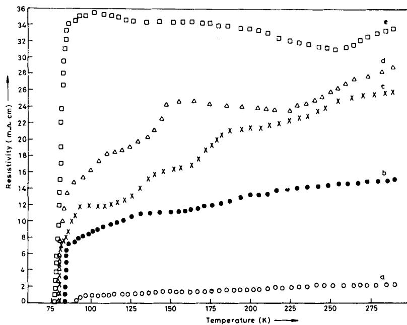
Figure 5. Resistivity vs temperature plot for \text{YBa}_{2-x}\text{K}_x\text{Cu}_3\text{O}_{7-\delta} , where x = (a) 0.2, (b) 0.4, (c) 0.6, (d) 0.8 and (e) 1.0.
