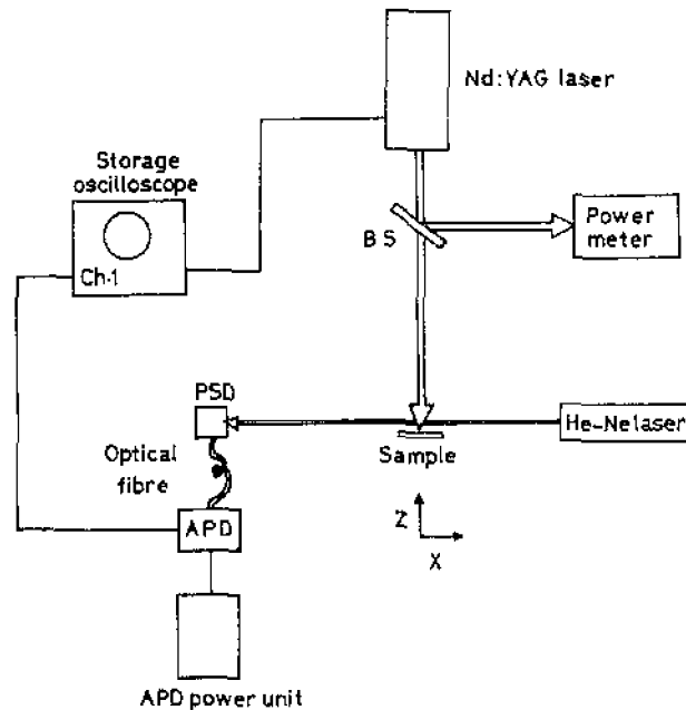
Figure 2. Schematic diagram of the experimental set-up.
