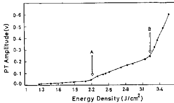
Figure 5. Plot of laser energy density vs PT amplitude for teflon in air.
