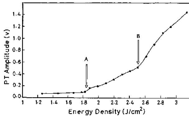
Figure 4. Plot of laser energy density vs PT amplitude for nylon in air.
