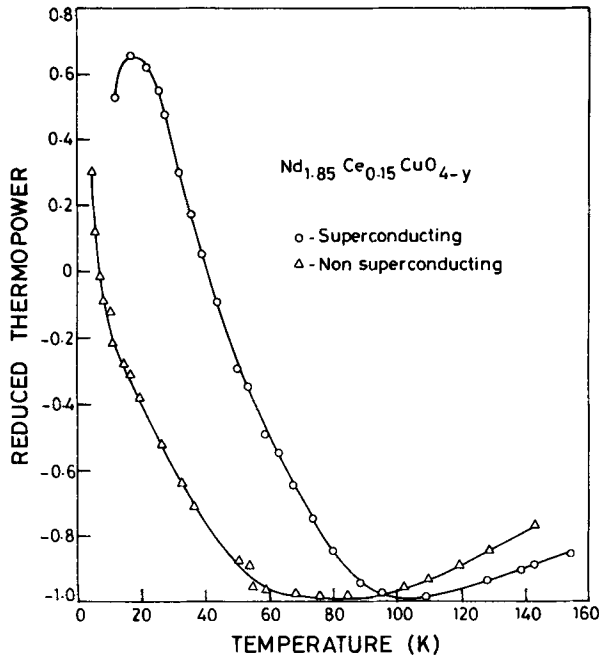
Figure 3. Thermopower vs temperature of \text{Nd}_{1.85}\text{Ce}_{0.15}\text{CuO}_{4-y} .
