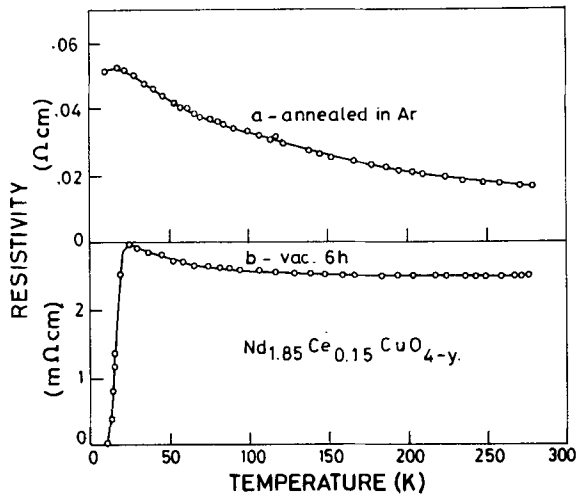
Figure 1. Resistivity vs temperature of \text{Nd}_{1.85}\text{Ce}_{0.15}\text{CuO}_{4-y} .
