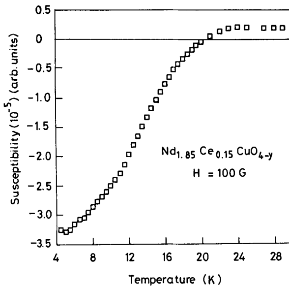
Figure 2. Susceptibility vs temperature of \text{Nd}_{1.85}\text{Ce}_{0.15}\text{CuO}_{4-y} .
