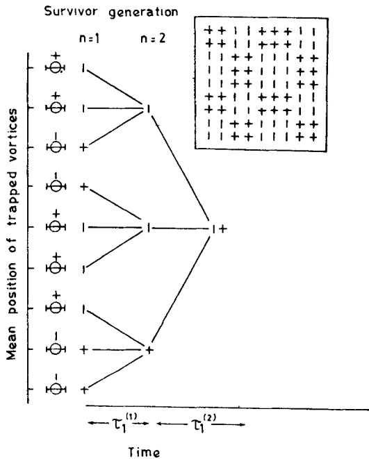
Figure 2. Hierarchical annihilation of mobile \pm 1 vortices with time, on a \pm \Phi flux fixed 1D flux pattern. (Inset: 2D vortex initial pattern, flux not shown).
