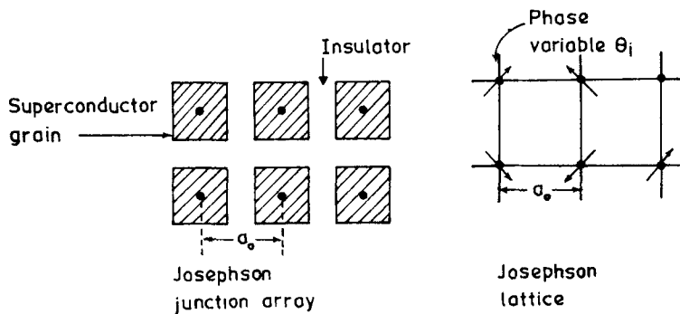
Figure 1. Josephson junction array and lattice model.
