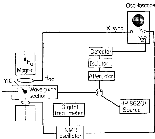
Figure 2. Experimental arrangement for non-resonant measurement of 4\pi M_s and g_{\text{eff}} of single crystal YIG spheres.
