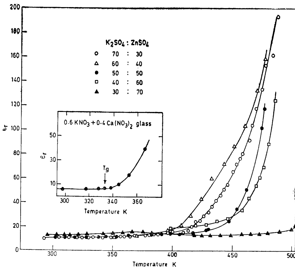
Figure 3. Behaviour of dielectric constant as a function of temperature for different glass compositions at 1 kHz. The corresponding T_g 's are ○ : 482 K; △ : 458 K; ● : 488 K; □ : 480 K; ▲ : 463 K. The inset of the figure corresponds to the behaviour \epsilon_r of a KNO_3 - Ca(NO_3)_2 glass at 1 kHz : data are from Howell et al 1974.
