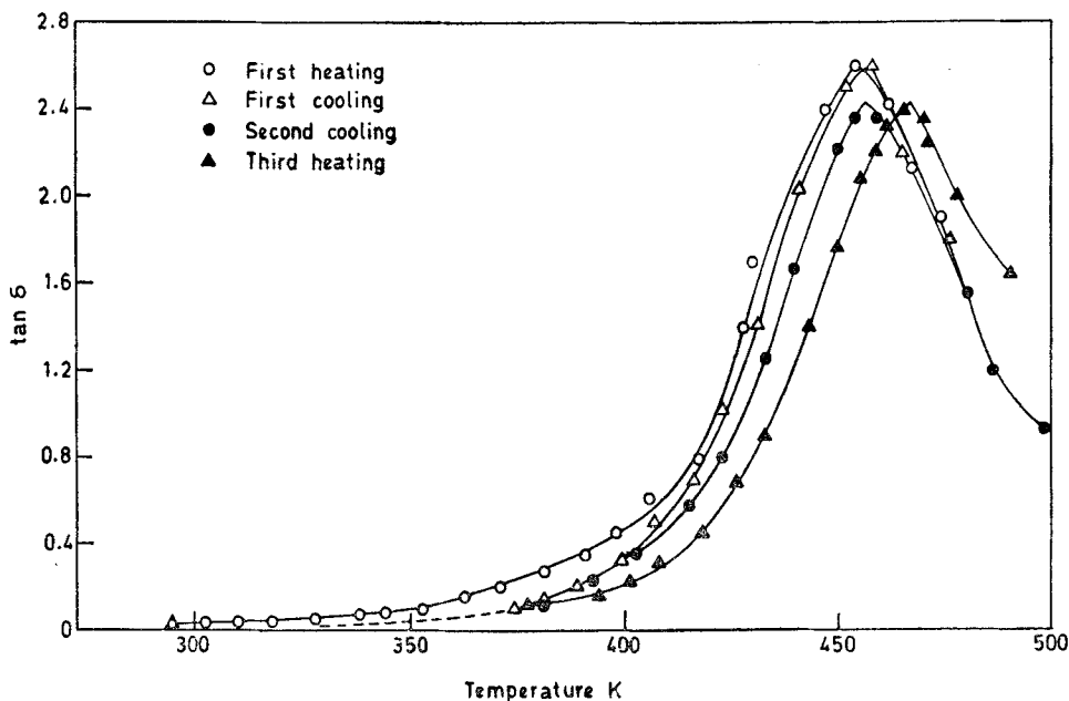
Figure 2. Effect of annealing on the behaviour dielectric loss curves in 50 : 50 : : \text{K}_2\text{SO}_4 : \text{ZnSO}_4 glass at 1 kHz.
