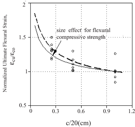
Figure 10. Comparison of ultimate strain with depth.
