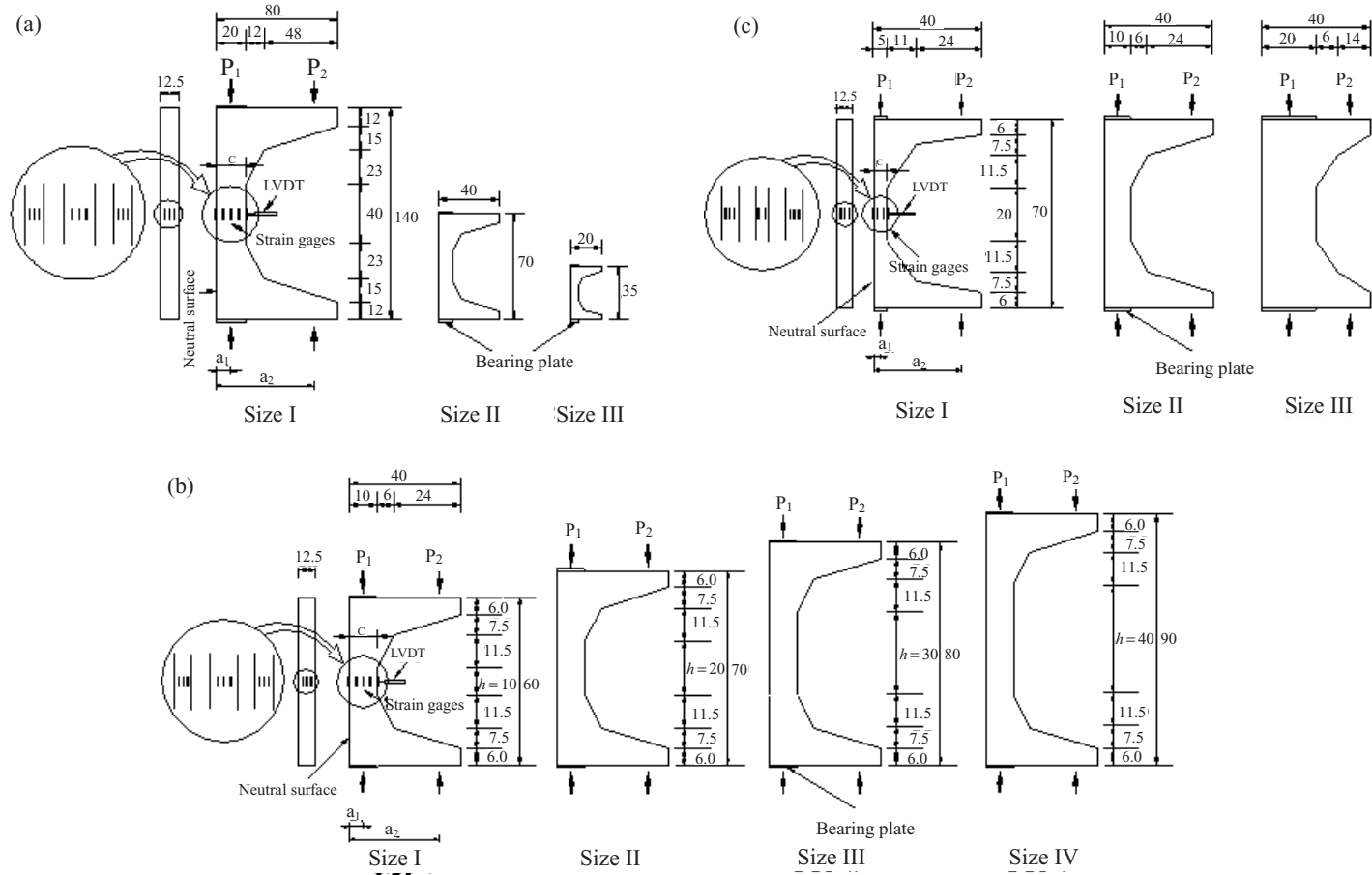
Figure 8. Size and shape of specimens (unit:cm). Effect of (a) size, (b) length and (c) depth.
