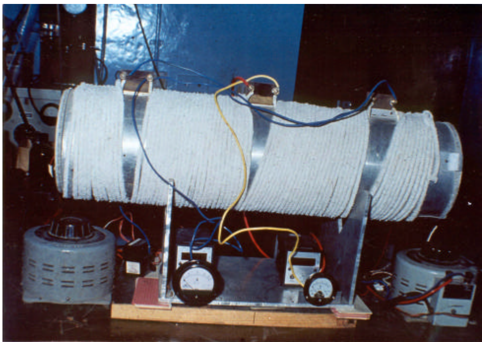
Figure 2. Photograph of cylindrical furnace for absorption spectral studies.
