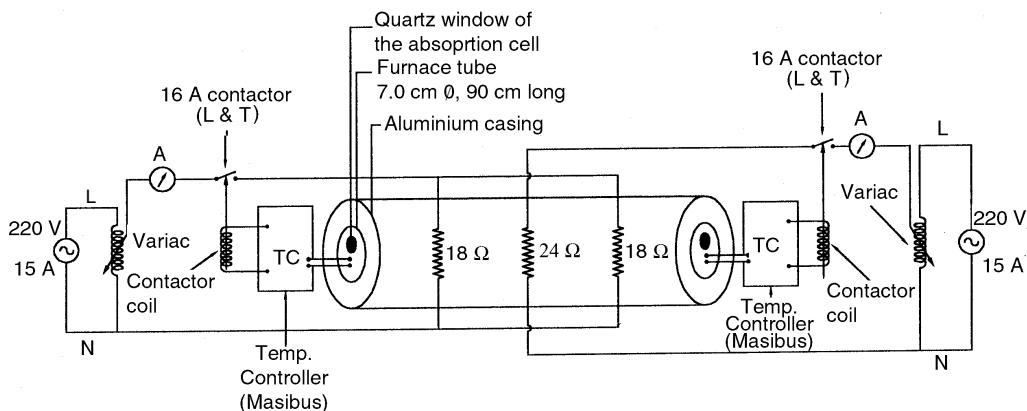
Figure 1. Circuit diagram of cylindrical furnace.
