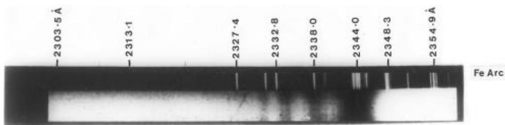
Figure 3. Absorption spectrum of I \leftarrow X band system of \text{Hg}_2 molecule at \sim 2345 \text{ \AA} .
