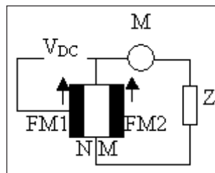
Figure 6. A normal metal is sandwiched between two ferromagnetic metals. A non-equilibrium polarization is induced into NM from FM1 on the left. One will measure a voltage or current on the meter M between NM and FM2 on the right.
