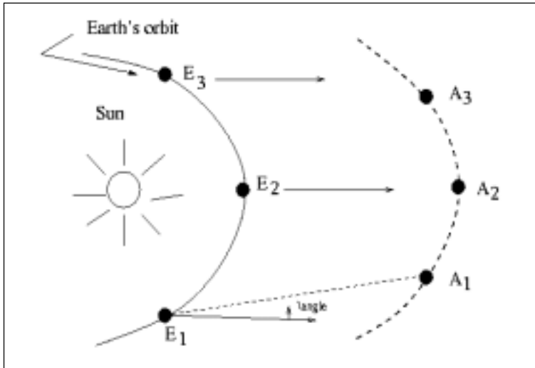
Figure 1. The (unknown) orbit of the asteroid is shown by dashed lines. At three different times t_1, t_2, t_3 , observations give the three directions (but not distances) of E_1A_1, E_2A_2 , and E_3A_3 . The earth's orbit E_1E_2E_3 is assumed known.
