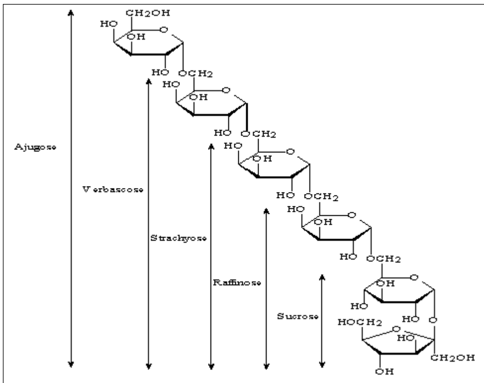
Figure 1. Structural relationship of the raffinose family sugars.
