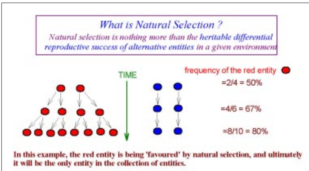
Figure 1. A schematic depiction of the basic notion of natural selection. Imagine a collection of two types of entities, red and blue. Initially, the collection consists of two each of the red and blue entities. Both kinds of entities last for one unit of time, and then disappear, after having made copies of themselves. They differ in the efficiency of making copies: the red entity makes two copies of itself at the end of one time unit, whereas the blue entity makes only one copy of itself. The figure shows how, as a consequence of the difference in the rate at which they make copies, the red entities come to outnumber the blue entities after a while. This is natural selection.
