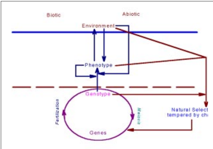
Figure 3. A more detailed view of evolution in living systems (the depiction is with diploid organisms in mind, but the general issues are the same for haploids as well). Below the dotted brown line is the genetic domain, and the dark violet circle represents the haploid-diploid-haploid cycling of genetic material through the alternation of meiosis and fusion. The blue arrows in the centre of the figure represent influences that play a role in the lifetime of an individual, whereas the brown arrows to the right of the figure represent influences on the evolution of the population of individuals.
