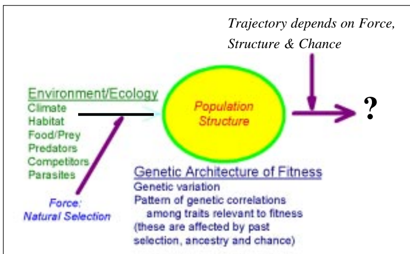
Figure 2. A simplistic view of adaptive evolution. The evolutionary trajectory of a population can be viewed as analogous to the trajectory of a body upon which a force acts. The evolutionary trajectory records how the phenotypic composition (and, therefore, the mean phenotype) of the population changes over time, and is the result of an interaction between the force of natural selection and the structure of the population. The force of natural selection is the resolution of the entire ecology of the organism into a net statement about which phenotypes are better able to survive and reproduce, while the structure of the population refers primarily to the way in which different traits relevant to fitness in that environment are genetically correlated with each other (modified from Fig. 1 in A Joshi 2000, J. Indian Inst. Sci. , 80: 25-37).
