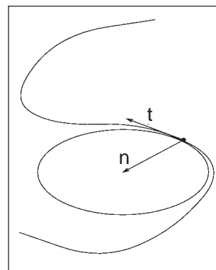
Figure 1 The osculating circle. ( t : tangent vector; n : normal vector.)
