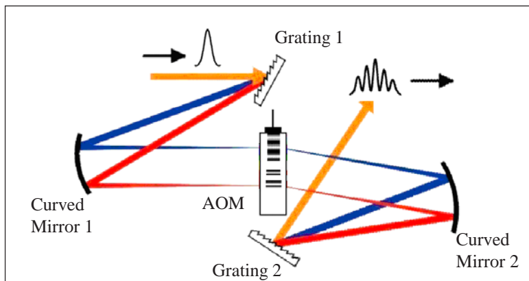
Figure 1. Schematic of an Acousto-Optic Modulator (AOM) based ultrafast pulse shaping technology that allows arbitrary programmable pulse shaping at high repetition rate of \sim 10^6 Hz.
