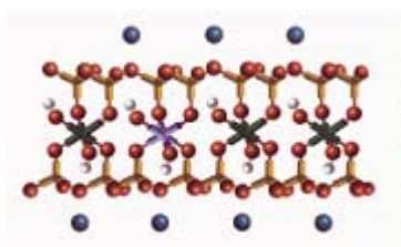
Figure A. MMT structure. Figure B. Intercalated structure Figure C. Exfoliated structure
