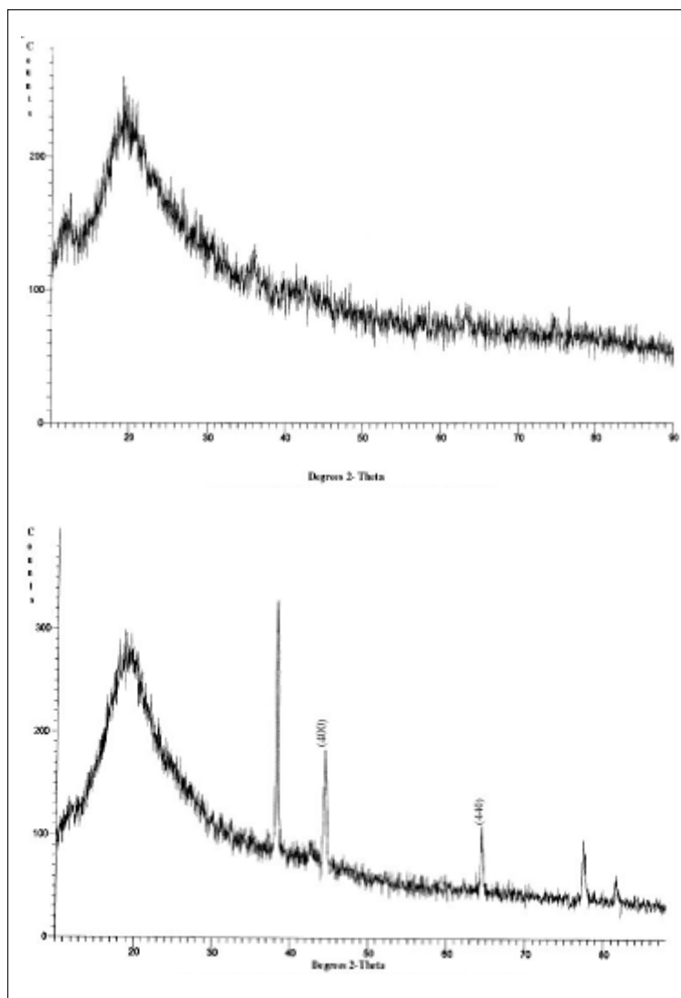
Figure 2. XRD pattern of (a) pure natural rubber (b) \gamma - \text{Fe}_2\text{O}_3 dispersed natural rubber.
