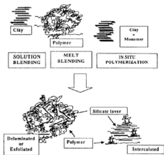
Figure D. Various methods used to prepare polymer layered-silicate nanocomposites
