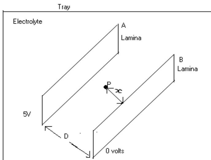
Figure 1. An electrolytic tank model with two brass laminas A and B separated by a distance D .
