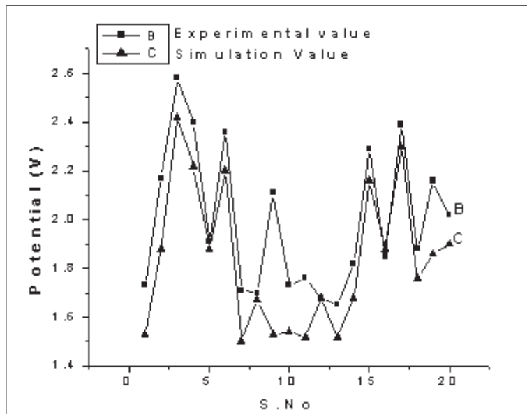
Figure 3. Comparison of experimental and simulation results (triangle).
