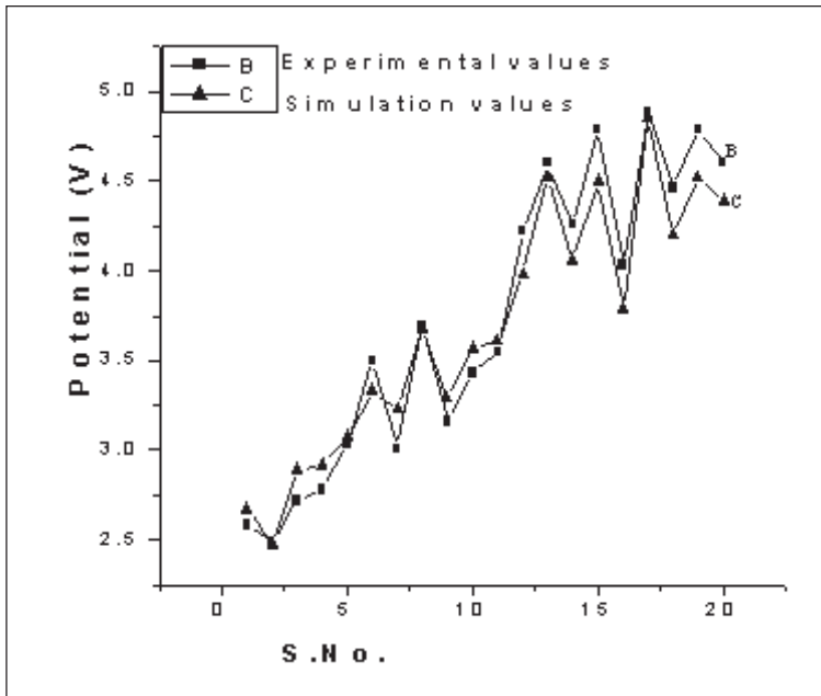
Figure 6. Comparison of experimental and simulation results (quadrilateral).
